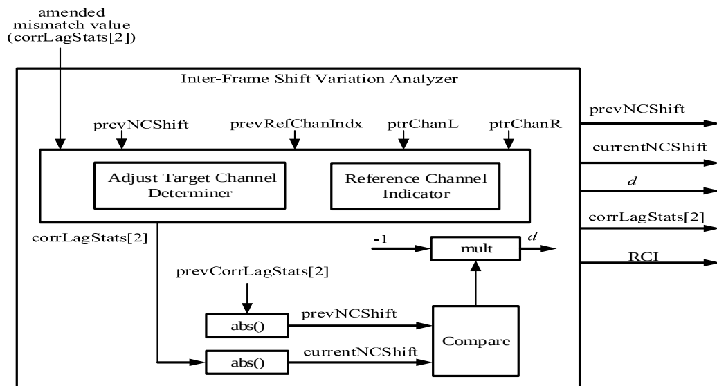
Figure 5-16: Block diagram of the Inter Frame Shift Variation Analyzer
