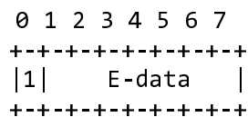
Figure A.3.3.3.3.1-1: E (Extra) byte structure
