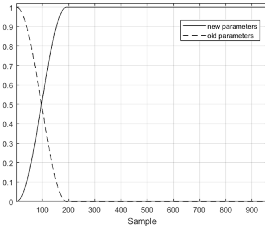
Figure 5.4-11: Cross-fading windows
