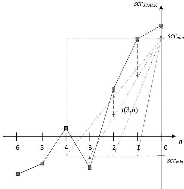
Figure 5.3-32: Rising-edge evaluation in the cross-talk detector in the TD stereo mode
