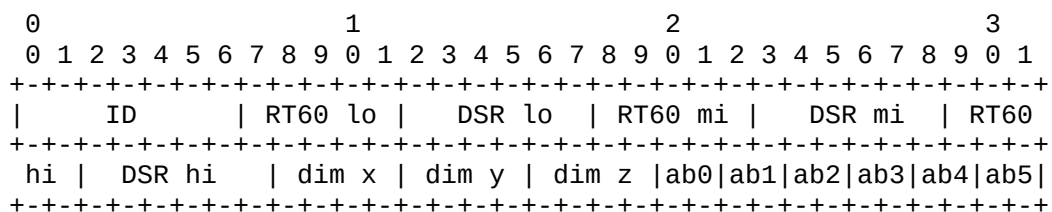
Figure A.3.5.6.2-3: Acoustic environment PI data frame (ACOUSTIC_ENVIRONMENT) containing a compact AE representation with late reverb and early reflection parameters.
