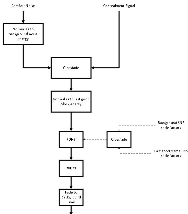
Figure 6.3-10: Fading to background noise in MDCT Stereo PLC
