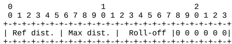
Figure A.3.5.6.4.7-1: ISM_DISTANCE_ATTENUATION PI data frame.
