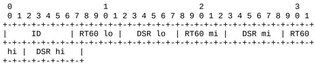
Figure A.3.5.6.2-2: Acoustic environment PI data frame (ACOUSTIC_ENVIRONMENT) containing a compact AE representation with late reverb parameters.
