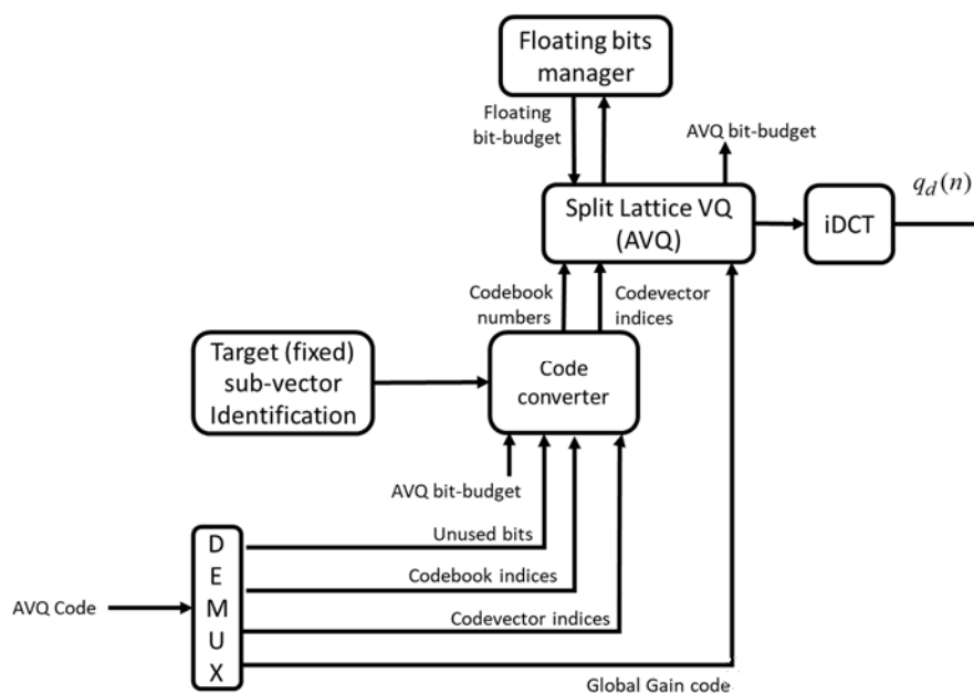
Figure 6.2-4: Overview of AVQ Bit Savings Decoder
