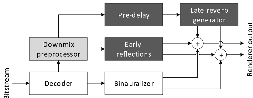
Figure 7.3-1: Synthetic reverb processing block diagram
