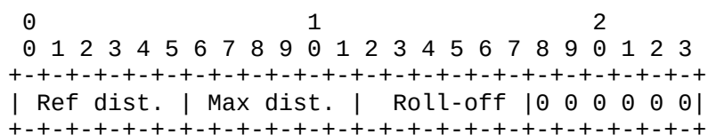
Figure A.3.5.6.4.7-1: ISM_DISTANCE_ATTENUATION PI data frame.
