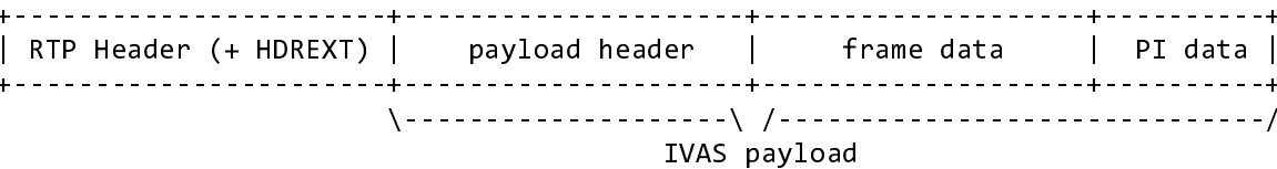
Figure A.3.3.2-1: RTP Header with IVAS payload structure
