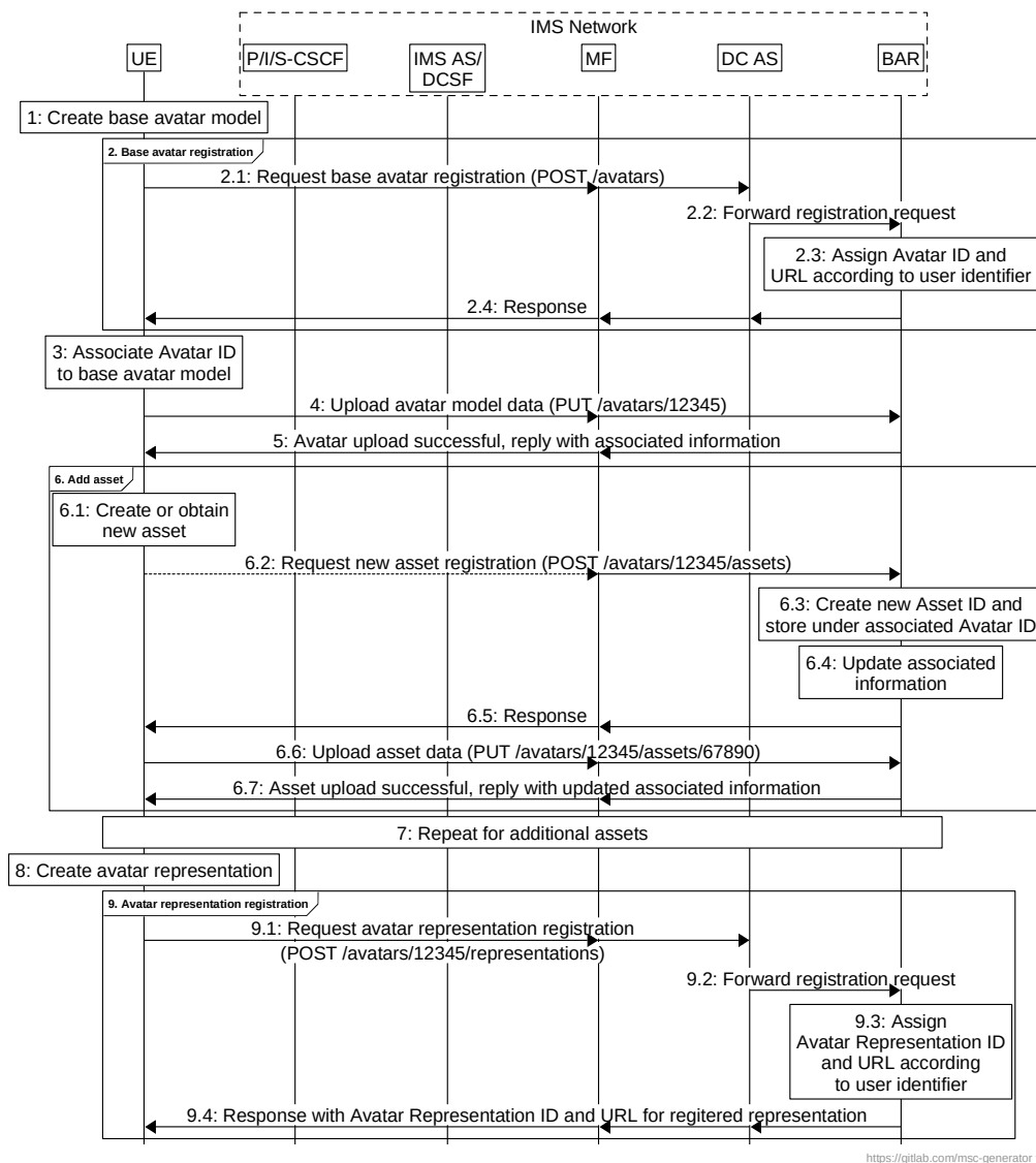
Figure A.2.2-1: Avatar management call flow via IMS network for registering and uploading base avatar model, avatar representation, and associated assets
