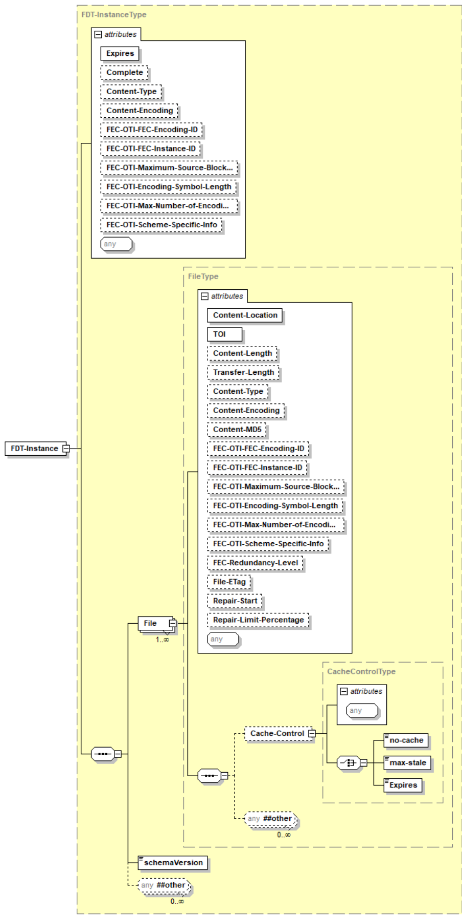
Figure L.6.1-1: Visualisation of consolidated FLUTE FDT schema
