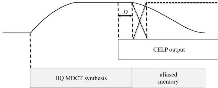
Figure 112a: Overlap-add in MDCT to CELP transition.
