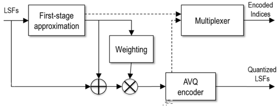
Figure 62: Principle of weighted algebraic LPC quantizer
