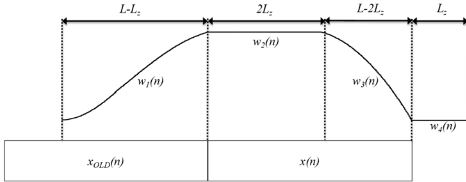
Figure 53: ALDO window
