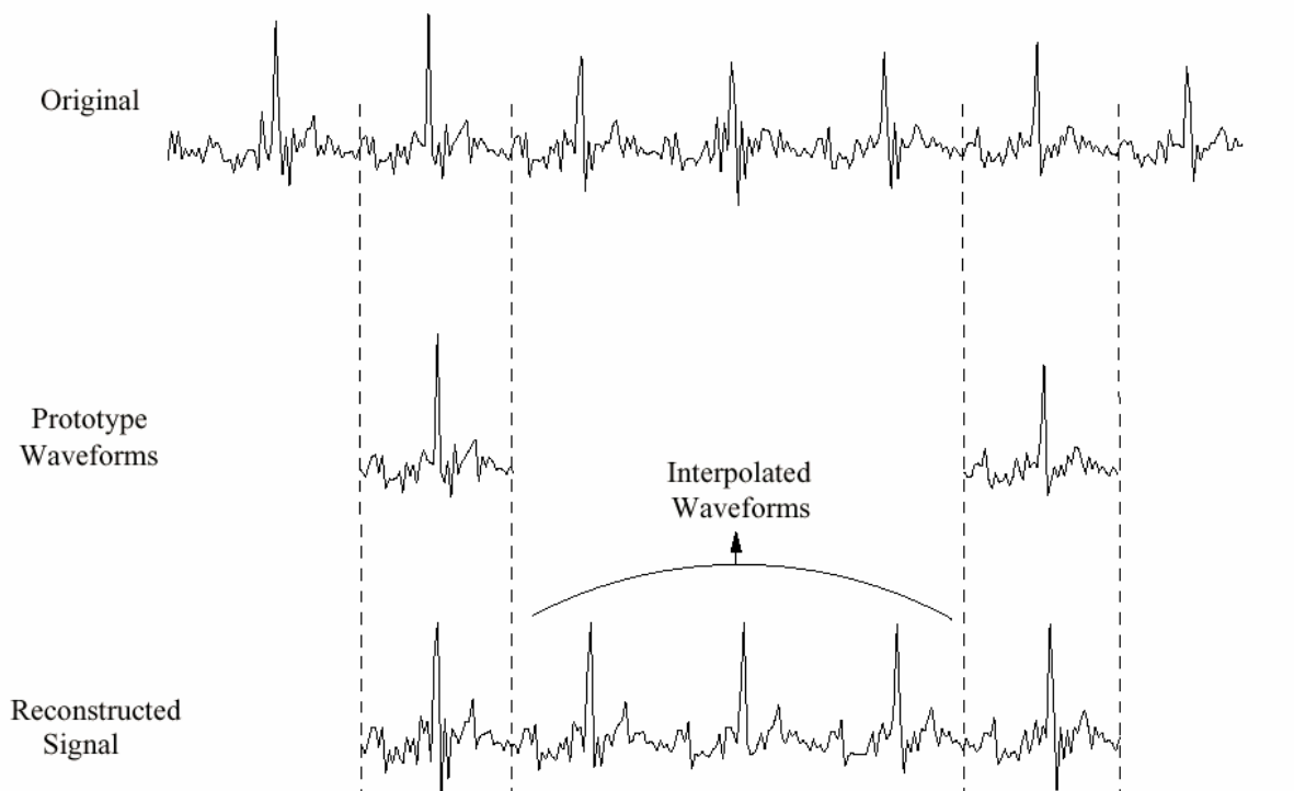
Figure 41: Illustration of principles of PPP coding [20]
