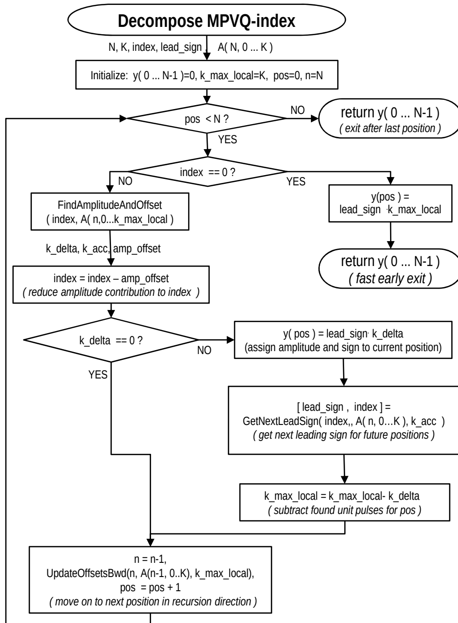
Figure 108: Detailed MPVQ-de-indexing
