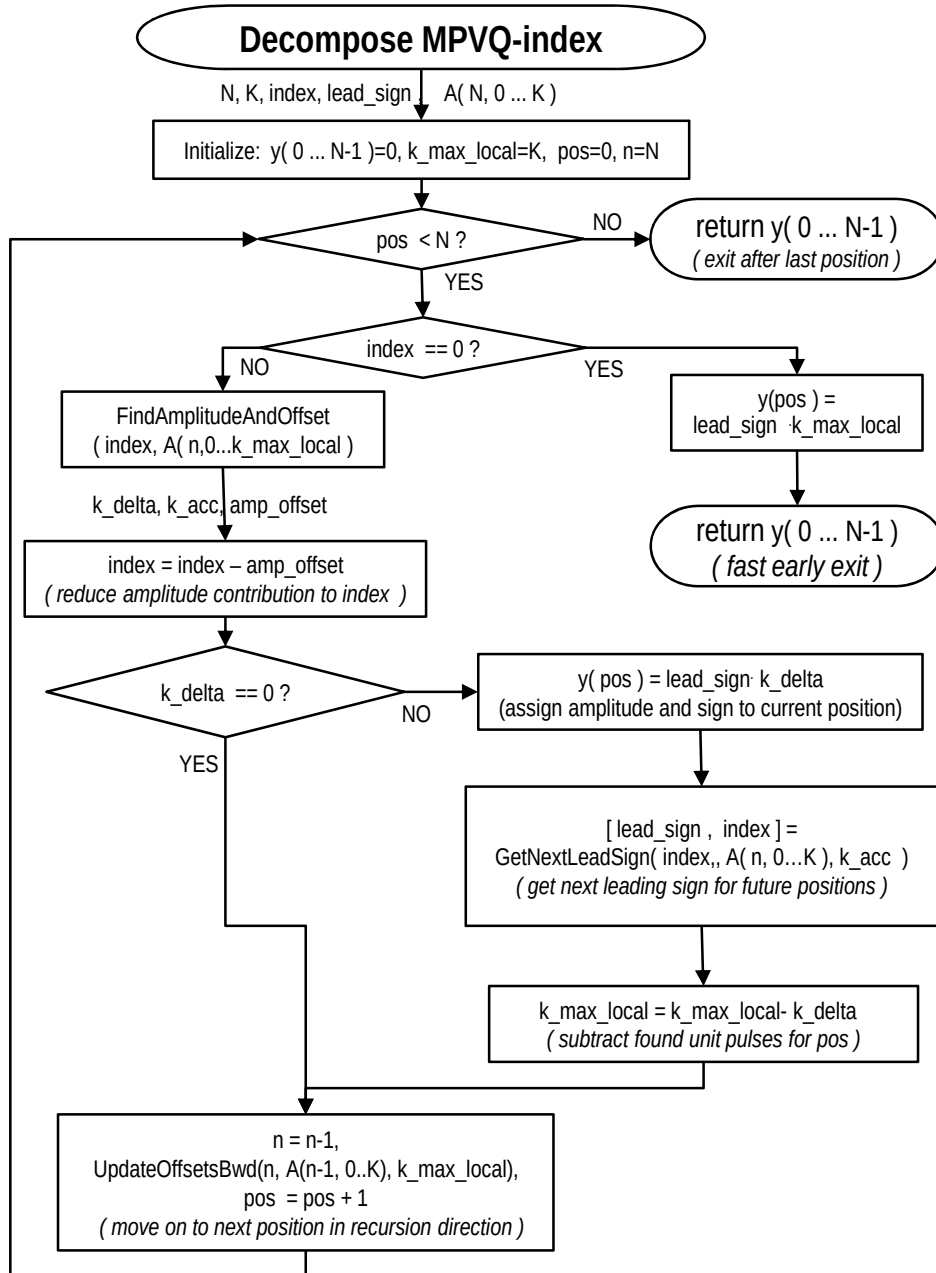
Figure 108: Detailed MPVQ-de-indexing
