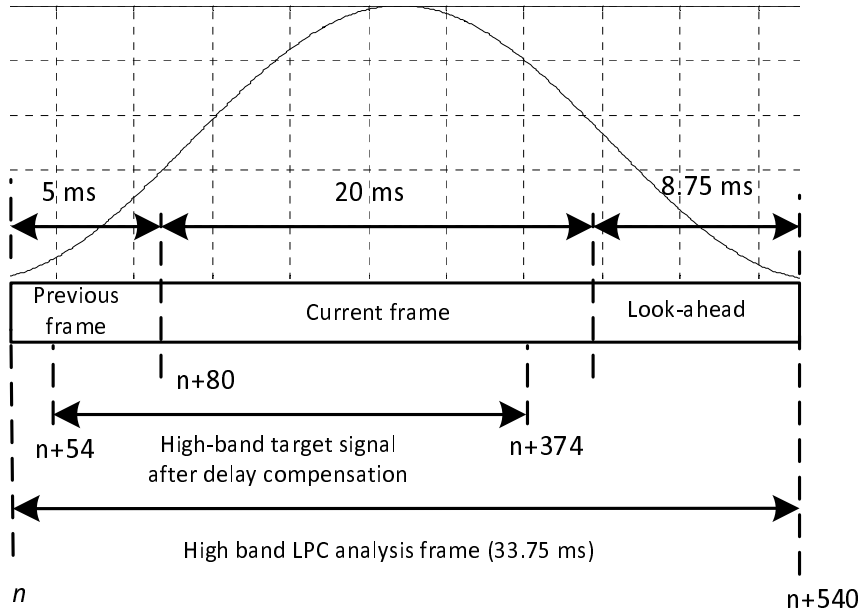
Figure 47: SWB Highband target signal buffers
