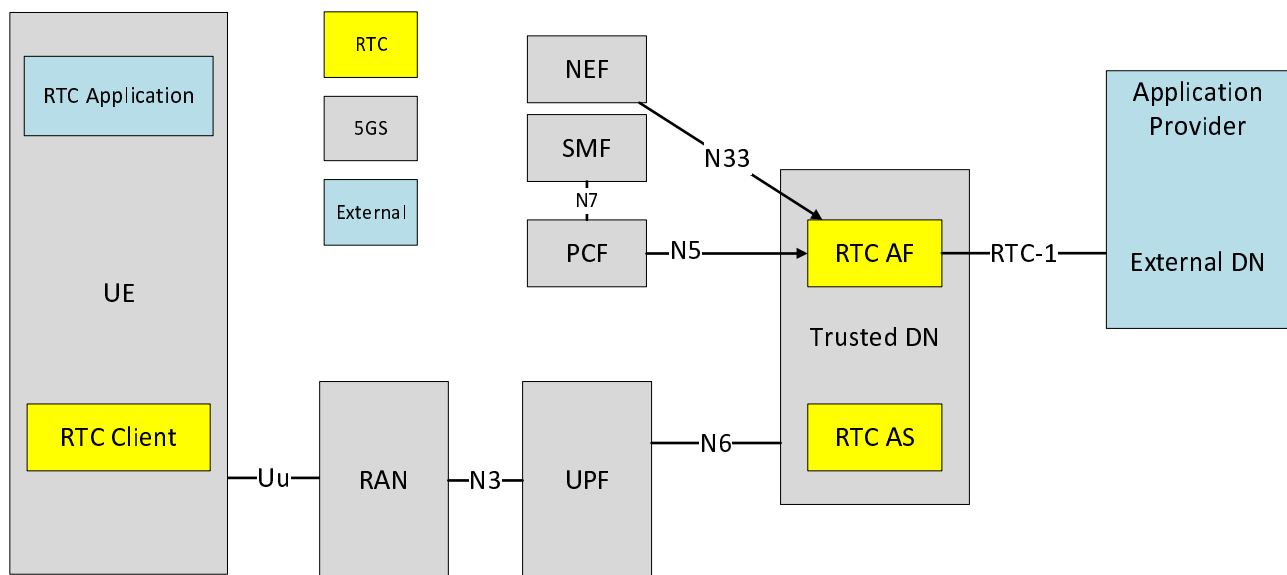
Figure 4.1.1-1: Real-time media communication (RTC) in 5G System
