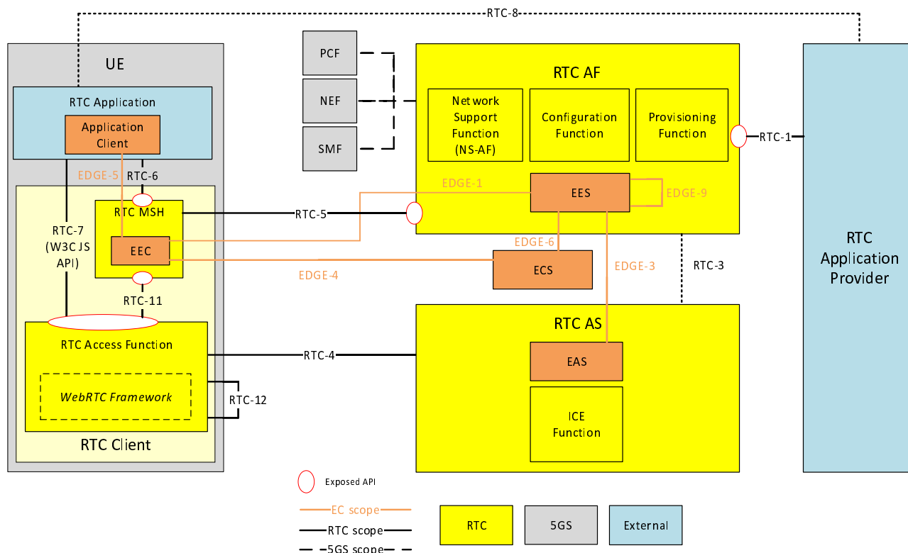
Figure 4.4.2-1: Edge-enabled RTC architecture
