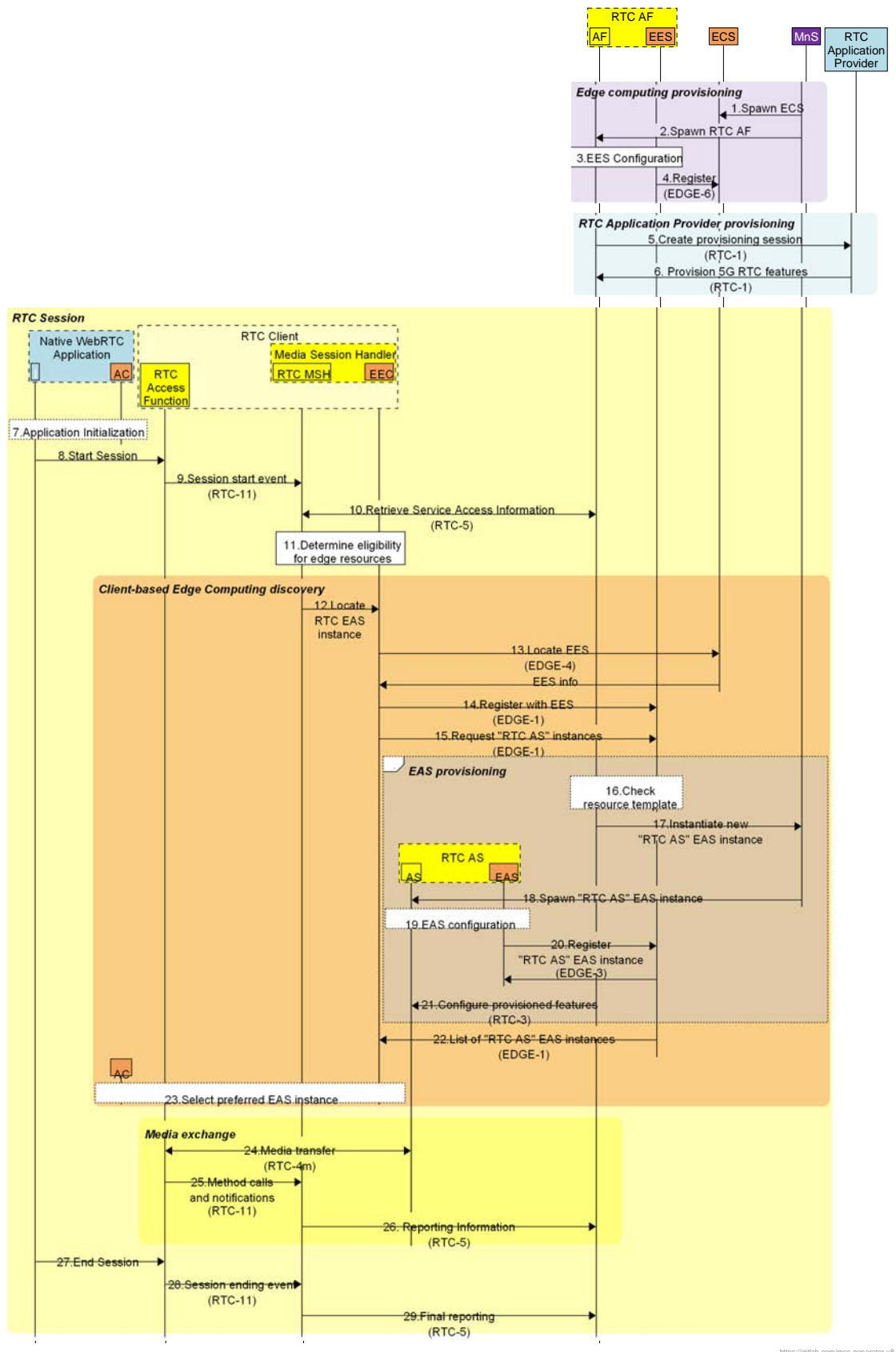
Figure 6.1-1. Client-driven management of RTC edge processing
