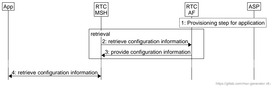
Figure 5.2.2-1: Configuration procedure
