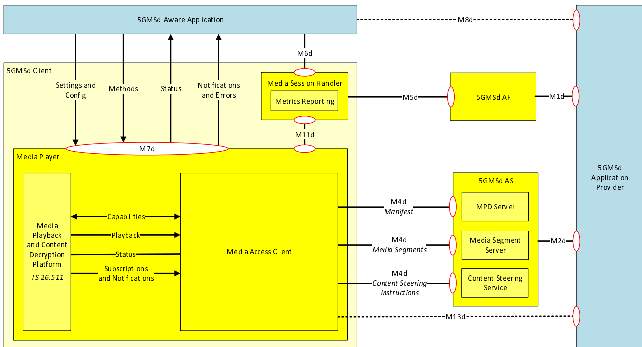
Figure 10.2-1: M4d usage for DASH distribution
