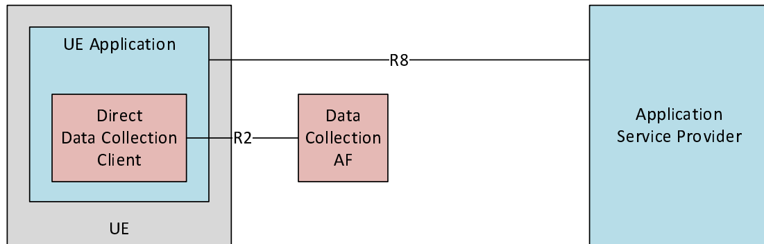
Figure A.6-1: Collaboration E with Data Collection Client deployed as part of the UE Application
