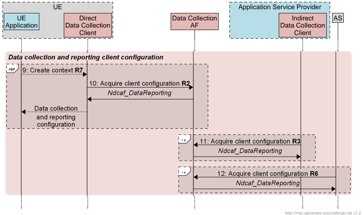
Figure 5.4-1: High-level procedures for data collection client configuration phase
