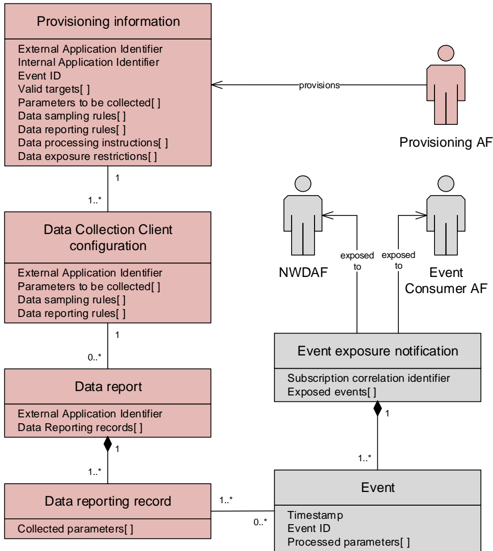
Figure 4.6.1-1: Static domain model
