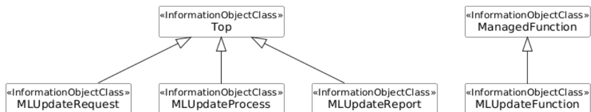
Figure 7.3a.4.1.2-1: Inheritance Hierarchy for ML update related NRMs
