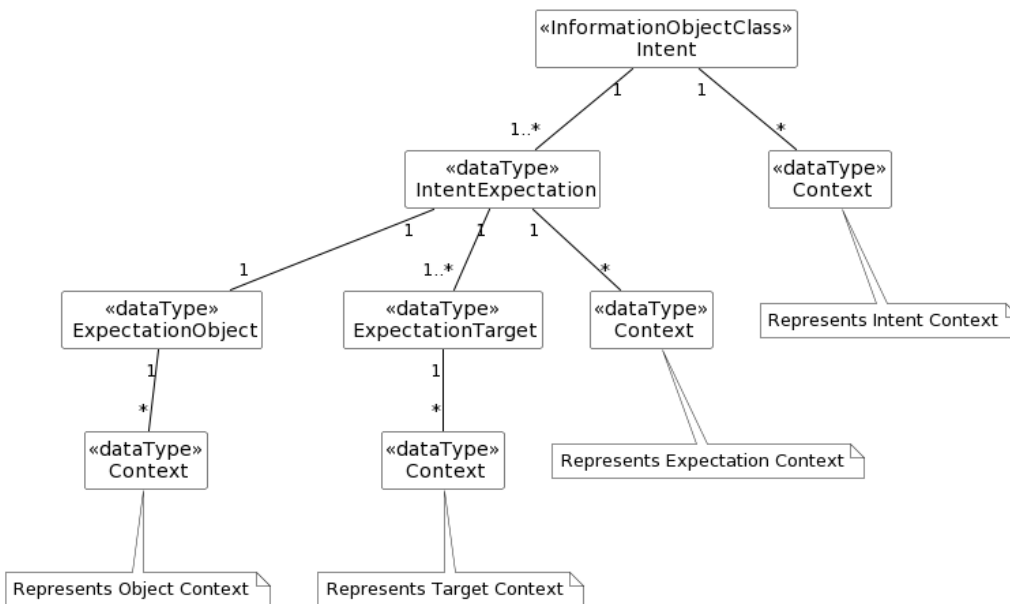
Figure 6.2.1.1.1-2: Relationship UML diagram for intent
