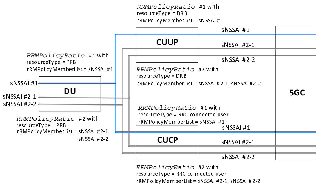
Figure 8.3.3-1: RRM policies for multiple network slice instances
