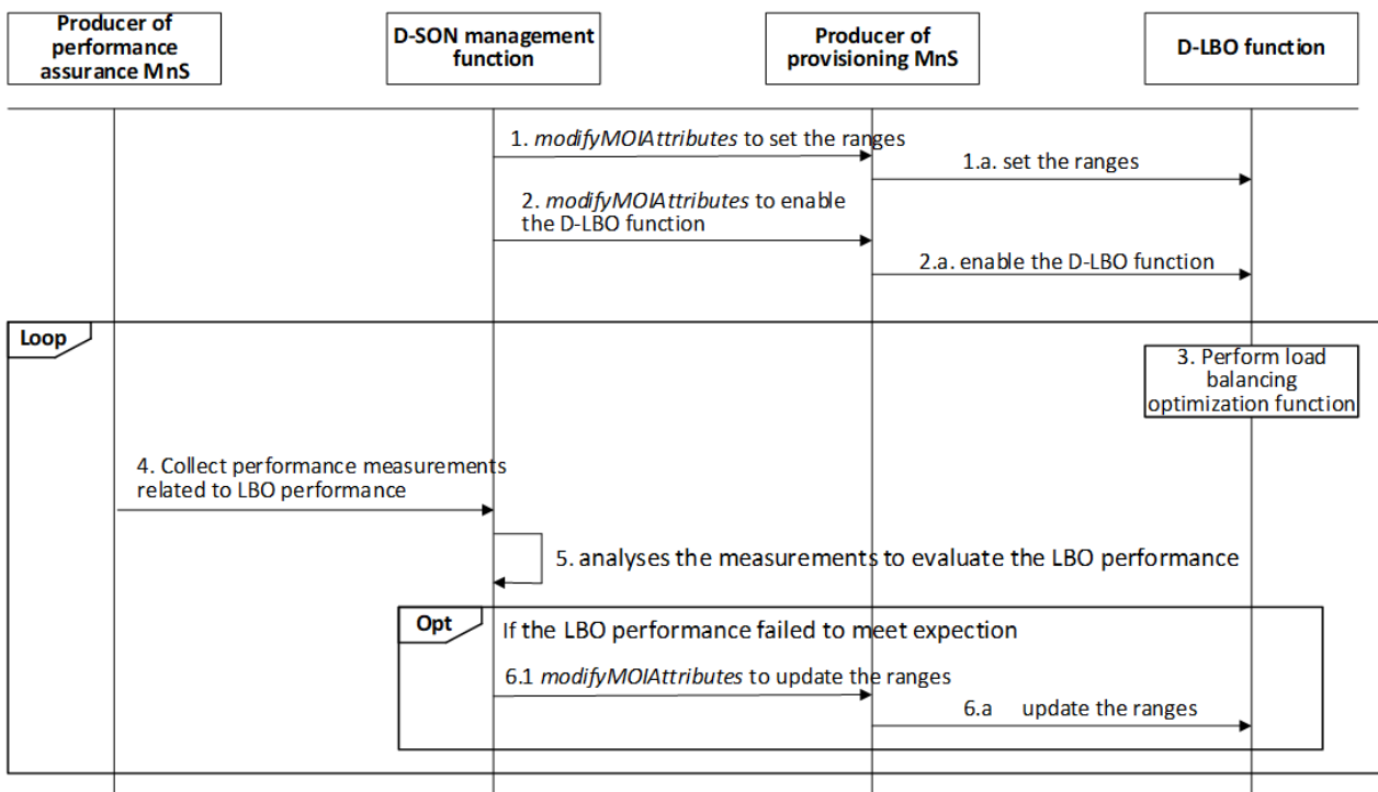
Figure 8.2.4-1: D-LBO procedure
