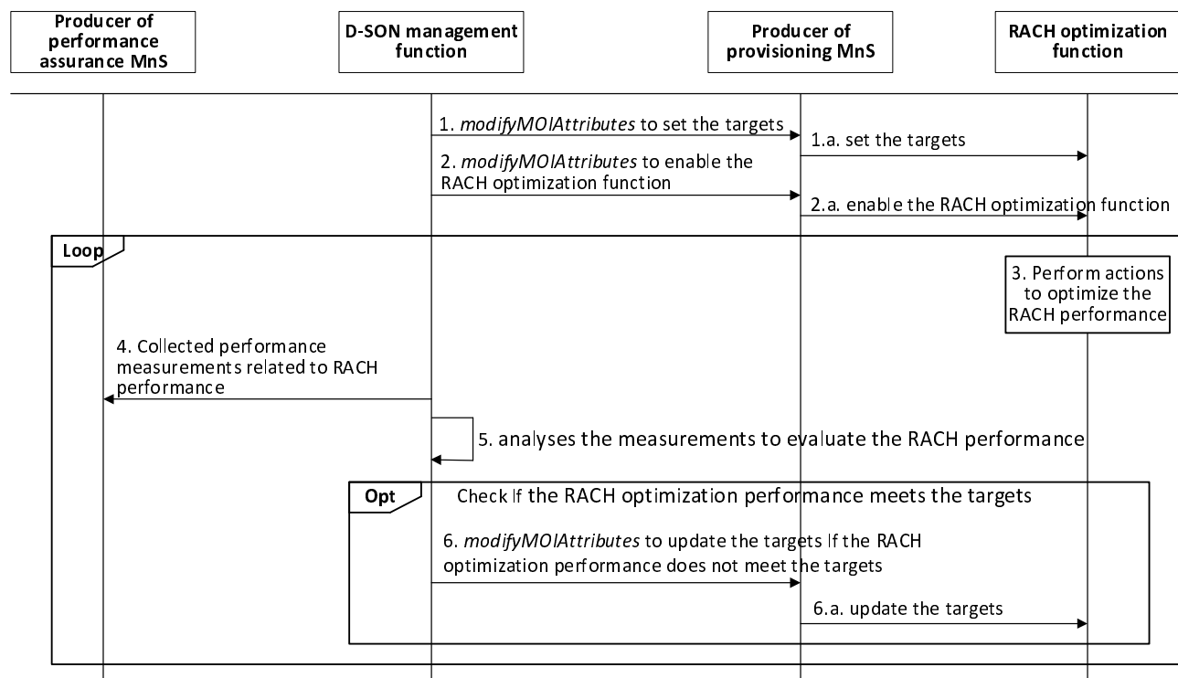
Figure 8.2.1-1: RACH Optimization procedure
