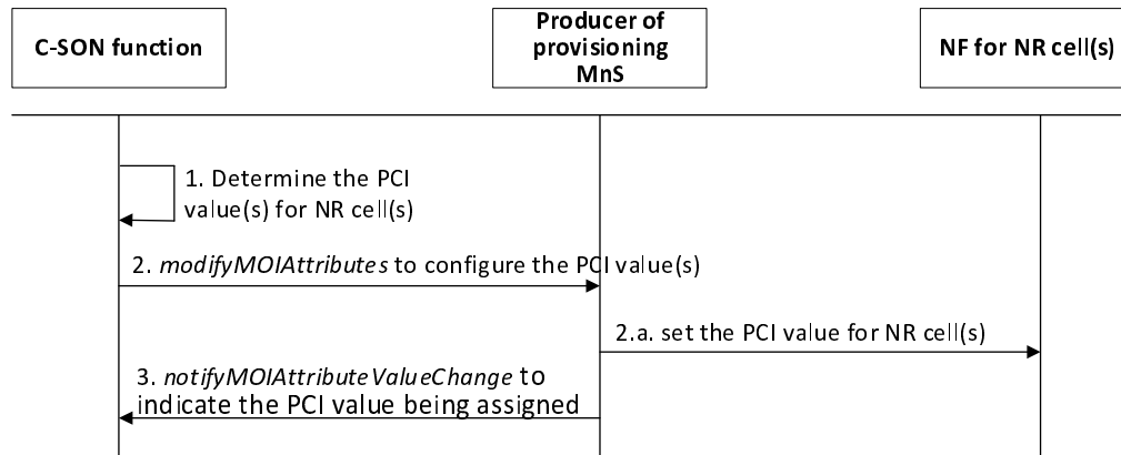
Figure 8.3.1.1-1: Initial PCI configuration procedure
