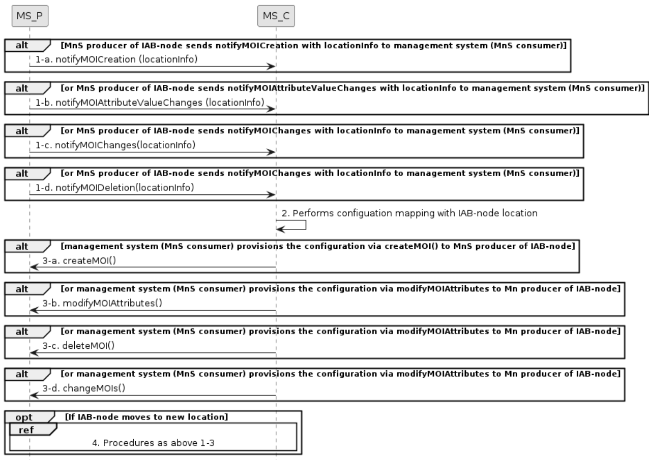
Figure 7.22-1 IAB-node configuration
