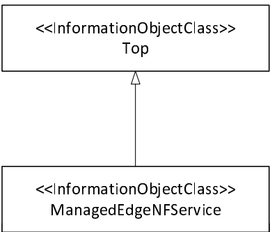
Figure 6.2.2-4 Inheritance hierarchy for ManagedEdgeNFService
