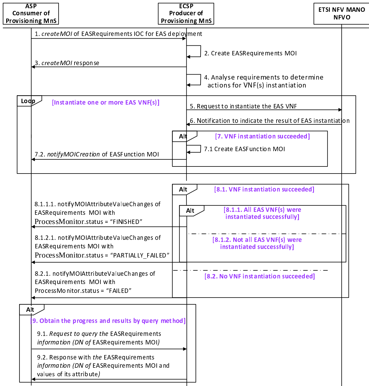
Figure 7.1.2.1.1-1: EAS deployment
