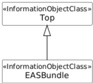
Figure 6.2.2-3 EASBundle Inheritance
