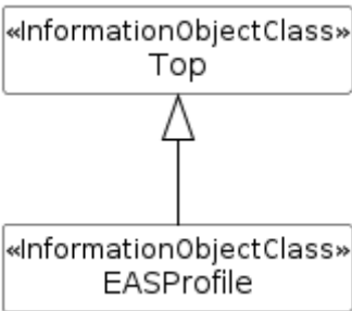
Figure 6.2.2-2: EASProfile Inheritance
