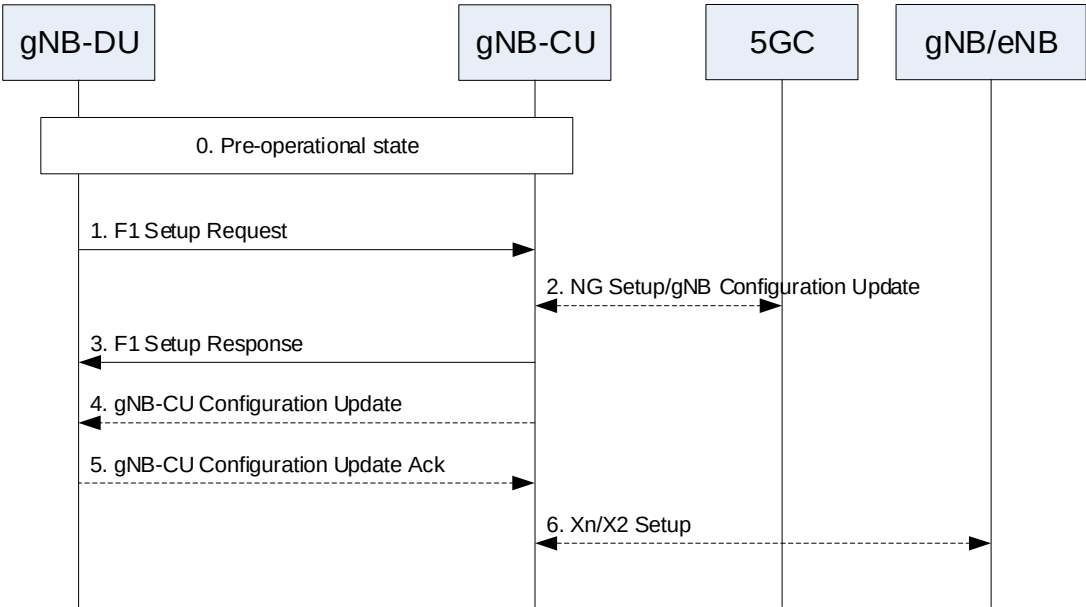
Figure 8.5-1: F1 startup and cell activation
