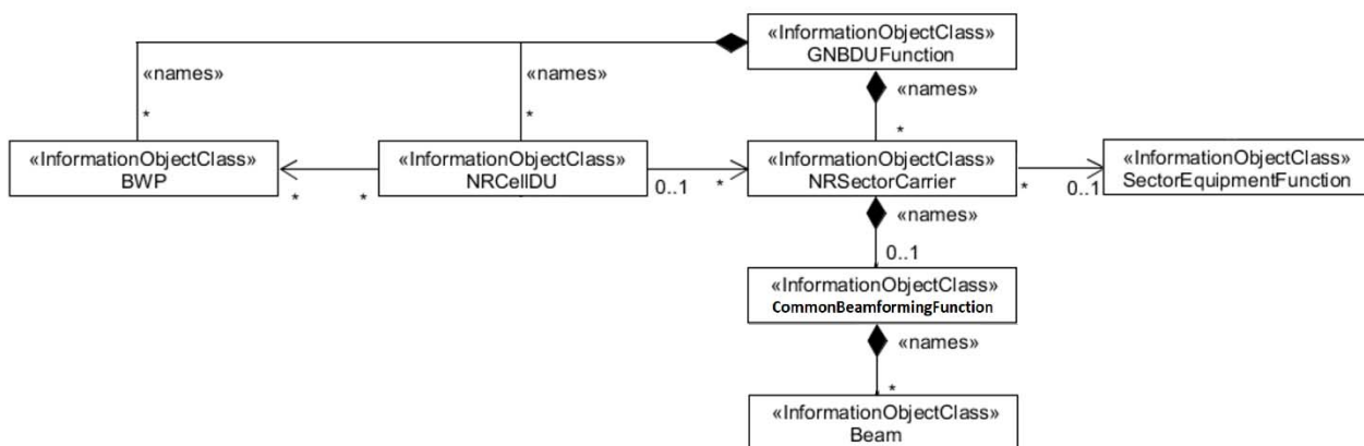
Figure 4.2.1.1-3: NRM for &lt;&lt;IOC&gt;&gt;NRSectorCarrier, &lt;&lt;IOC&gt;&gt;SectorEquipmentFunction and &lt;&lt;IOC&gt;&gt;BWP for all deployment scenarios
