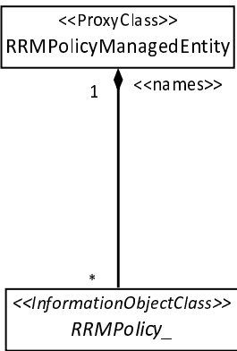
Figure 4.2.1.1-6: NRM fragment for abstract RRM Policies
