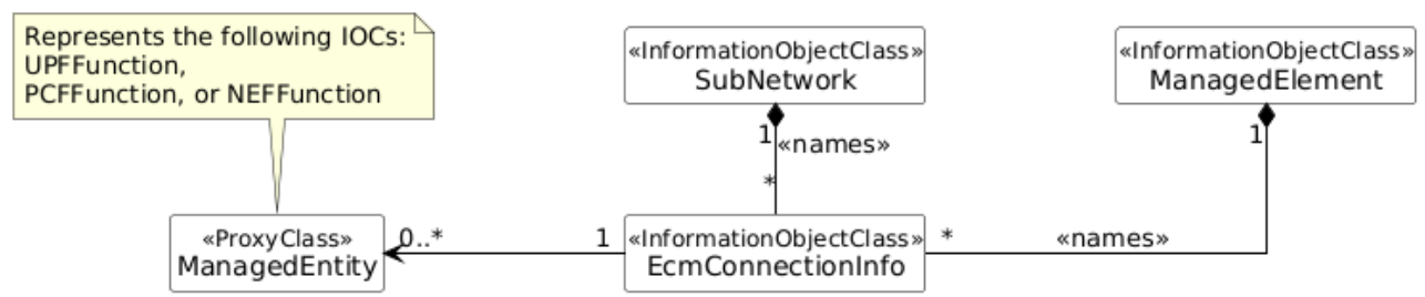
Figure 5.2.1.1-25: EcmConnectionInfo NRM
