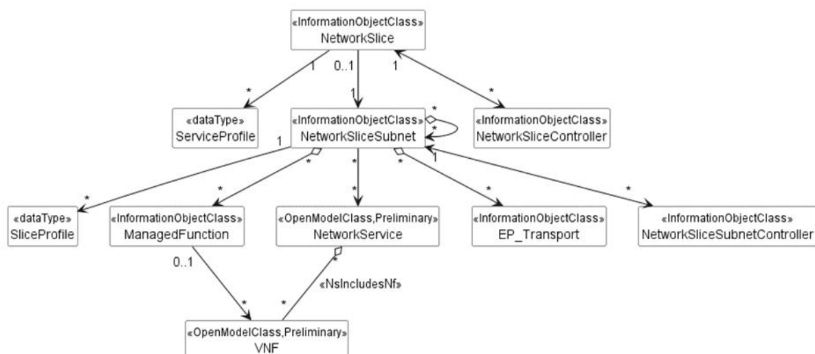
Figure 6.2.1-1: Network slice NRM fragment relationship
