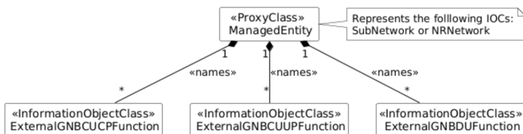
Figure 4.2.1.1-22: NRM fragment for ExternalGNBCUCPFFunction, ExternalGNBCUUPFunction and ExternalGNBDUFunction
