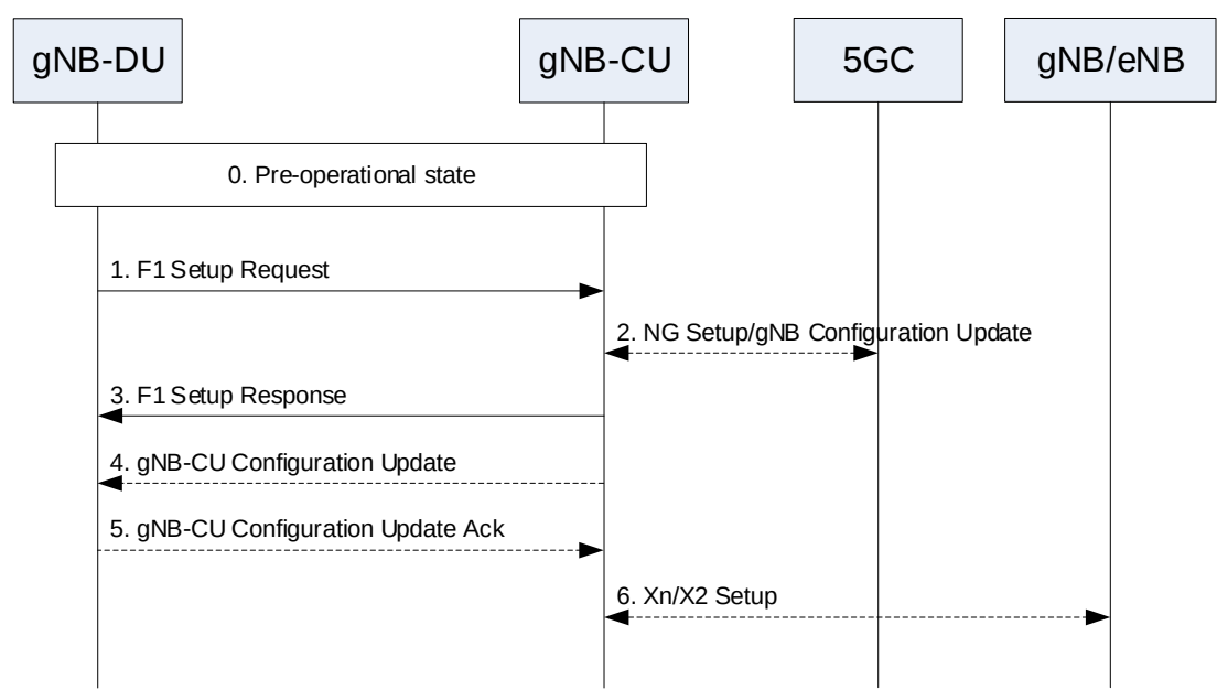
Figure 8.5-1: F1 startup and cell activation
