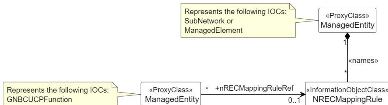
Figure 4.2.1.1-23: NRM fragment for energy cost mapping rule
