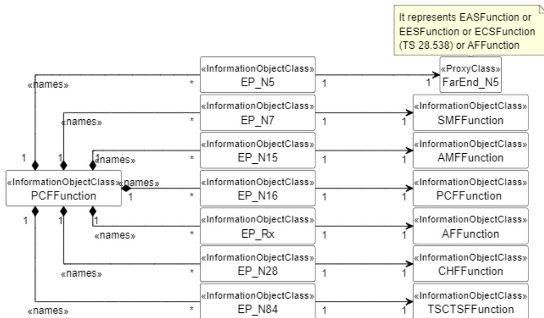
Figure 5.2.1.1-6: Transport view of PCF NRM
