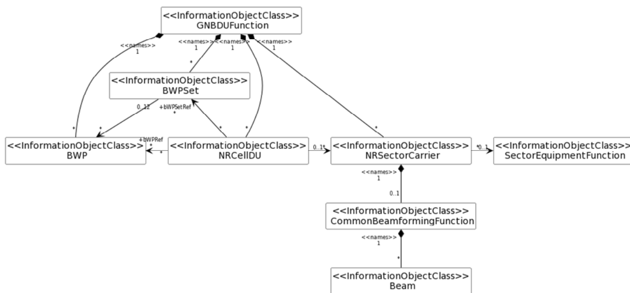
Figure 4.2.1.1-3: NRM for <<IOC>>NRSectorCarrier, <<IOC>>BWP, <<IOC>>SectorEquipmentFunction and <<IOC>> BWPSet for all deployment scenarios
