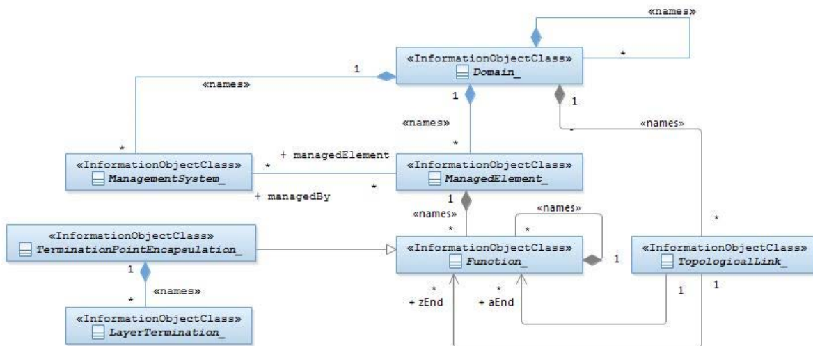
Figure 1: Class diagram
