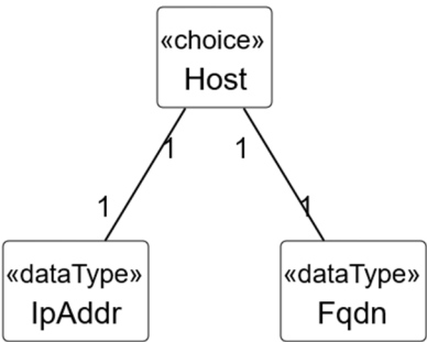
Figure 4.3.71.1-1 alternative dataType to this <<choice>>
