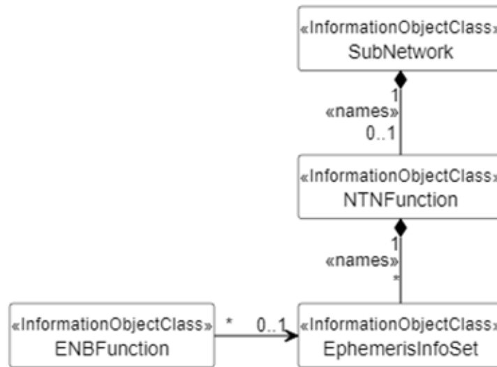
Figure 4.2.1-9: IoT-NTN related Attributes NRM IOCs
