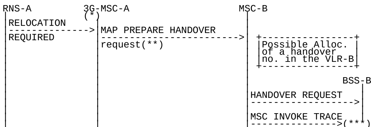
Figure 21b: Signalling for Basic Inter-MSC Handover initiation (MSC invoke trace message transferred)
