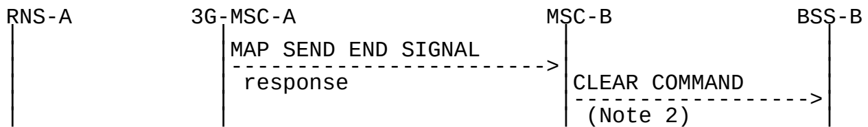
Figure 25: Signalling for Basic Inter-MSC Handover completion (Positive outcome)
