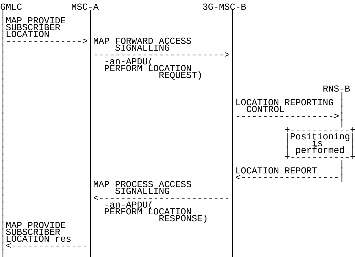
Figure 65b: Signalling for a completed Location Acquisition procedure
