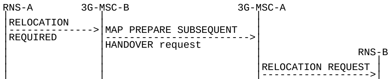
Figure 55: Signalling for Subsequent Inter-MSR Relocation back to 3G_MSC-A initiation
