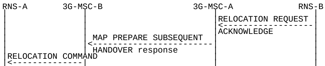
Figure 56: Signalling for Subsequent Inter-MSR Relocation back to 3G_MSC-A execution (Positive outcome)
