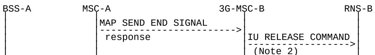
Figure 41: Signalling for Basic Inter-MSC Handover completion (Positive outcome)
