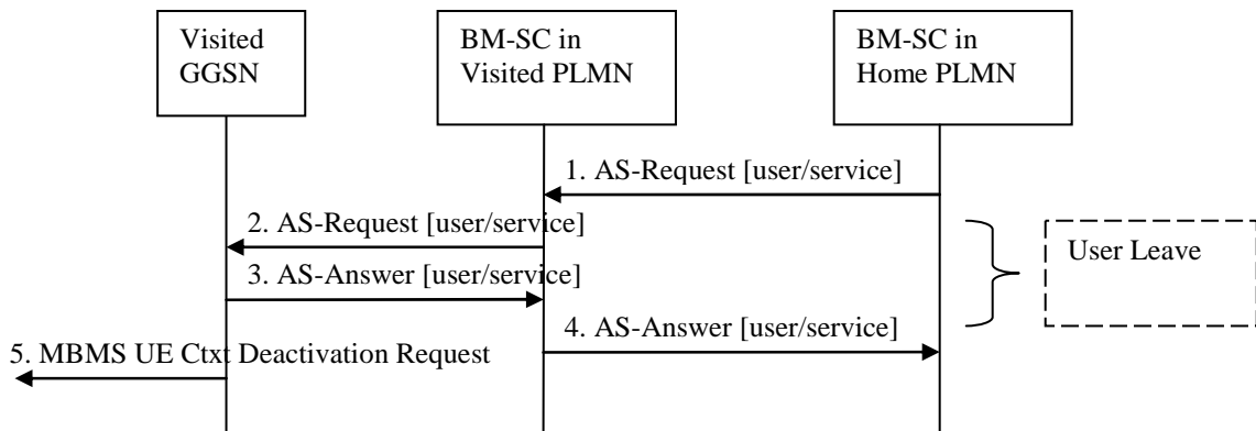
Figure 32b: BM-SC in the home PLMN initiated MBMS multicast service deactivation procedure
