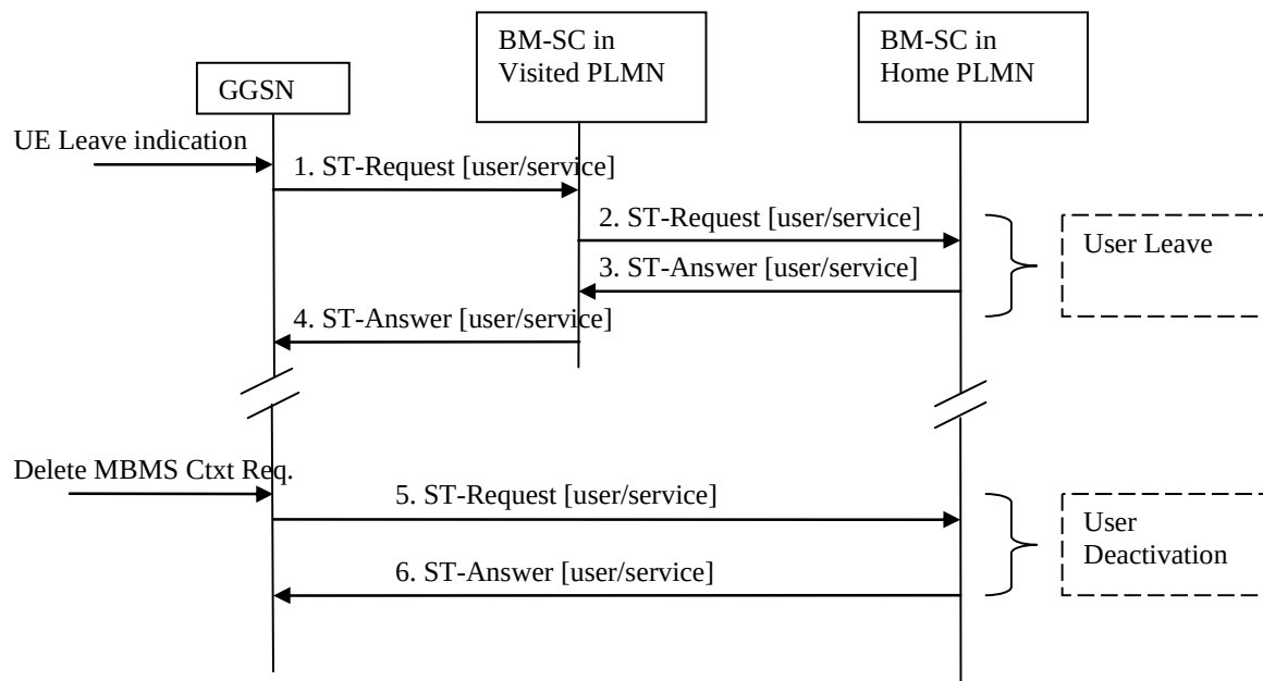
Figure 30a: Deactivation of an MBMS multicast service in roaming scenario with service provided in the home PLMN
