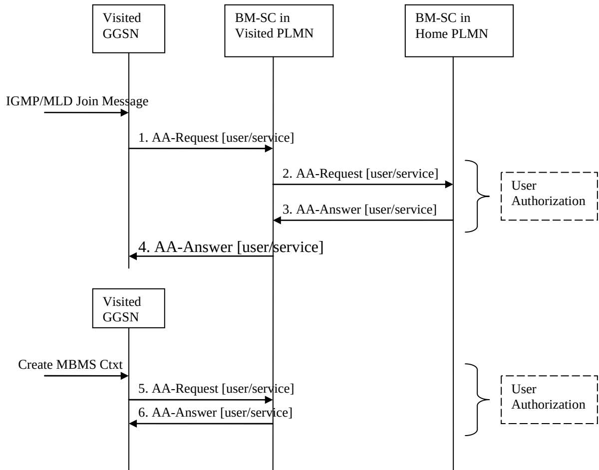
Figure 29a: Activation of an MBMS multicast service in roaming scenario with service provided in the visited PLMN
