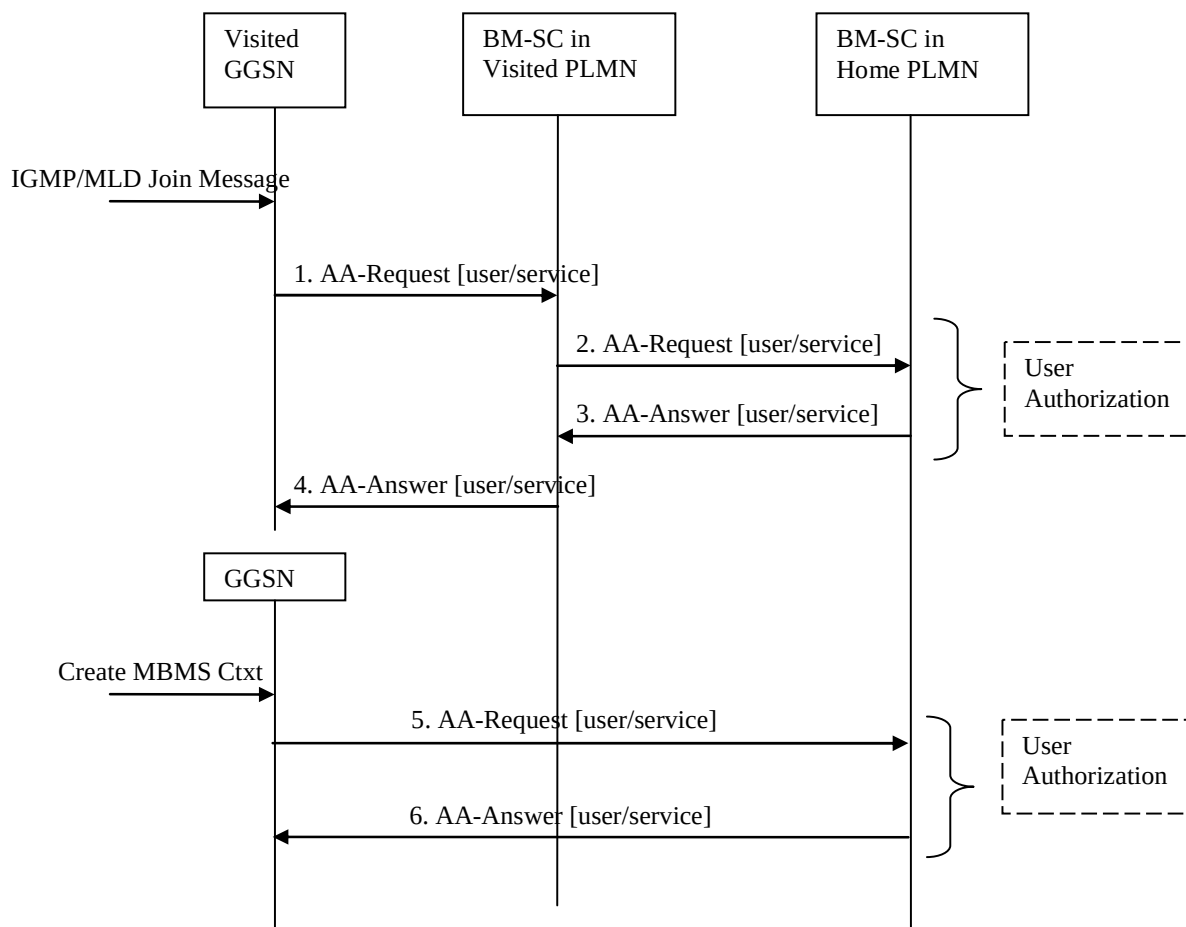
Figure 28: Activation of an MBMS multicast service in roaming scenario with service provided in the home PLMN
