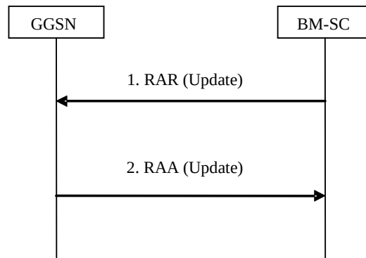
Figure 27a: MBMS Session Update procedure
