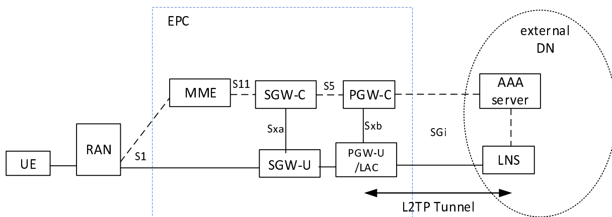
Figure 11f: L2TP Tunnel between CUPS and external DN
