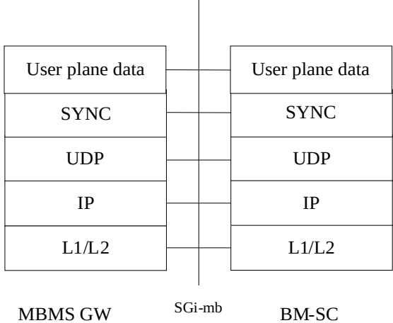
Figure 16l: The user plane protocol stacks of MBMS GW for interworking with BM-SC for broadcast
