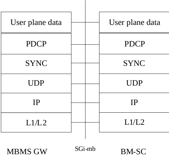
Figure 16k: The user plane protocol stacks of MBMS GW for interworking with BM-SC for multicast
