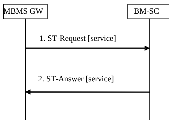
Figure 20.3.4.1: MBMS session termination
