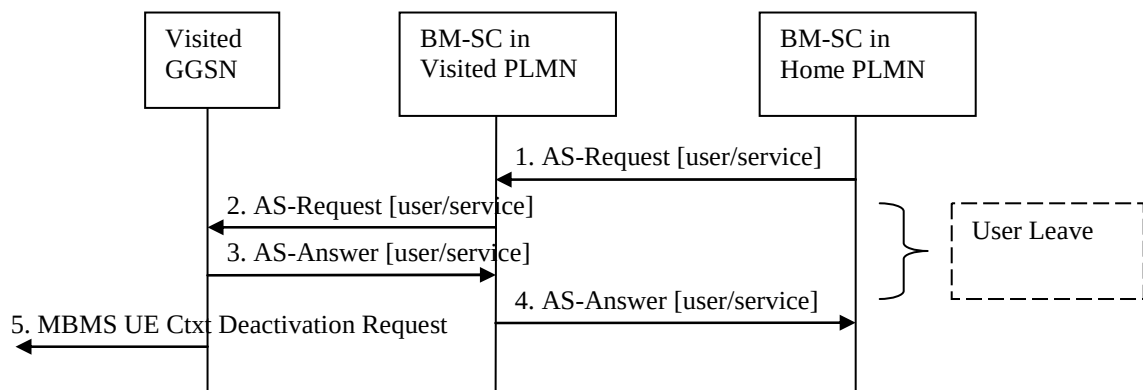
Figure 32b: BM-SC in the home PLMN initiated MBMS multicast service deactivation procedure
