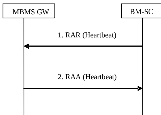
Figure 20.3.5.1: MBMS Heartbeat procedure initiated by the BM-SC
