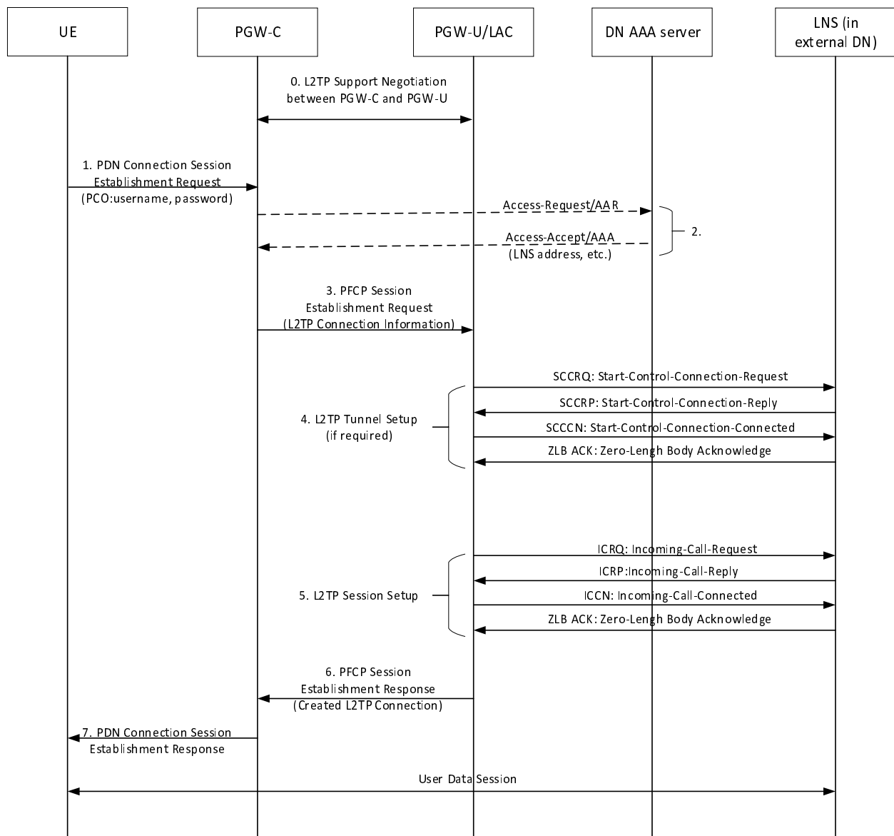
Figure 11g: L2TP connection procedures between CUPS and external DN
