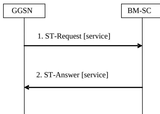
Figure 36: Broadcast session termination
