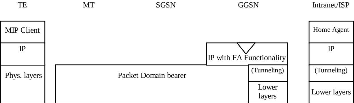
Figure 11d: Protocol stacks for user access with MIP
