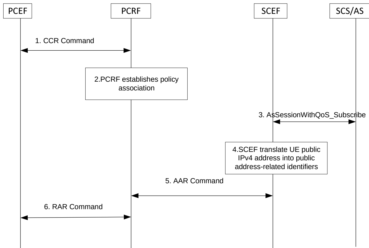
Figure L.2-1: SCEF translate public IPv4 address to public address-related identifier in IP domain
