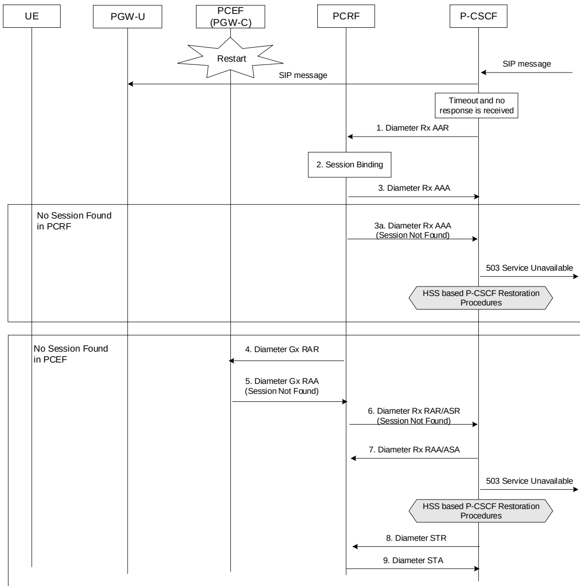
Figure B.9.2.1: P-CSCF initiated EPC Health Monitoring after PGW-C Failure
