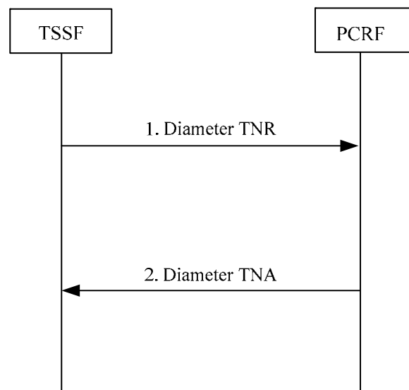
Figure 4.9.4.1: St notification initiated by the TSSF
