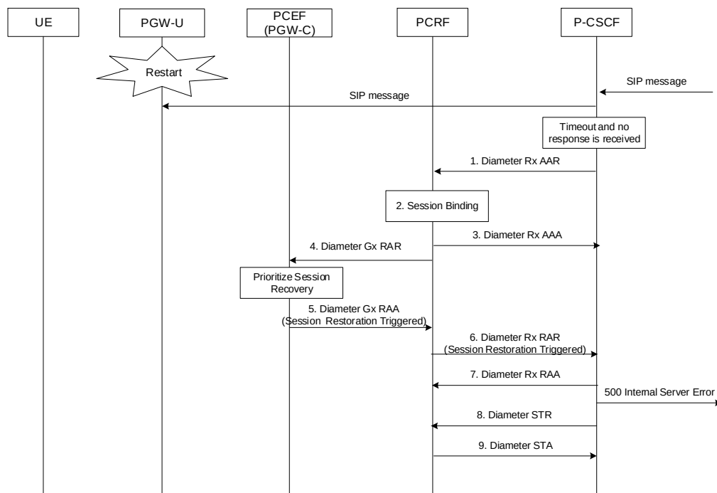
Figure B.9.1.1: P-CSCF initiated EPC Functions Health Monitoring and PGW-U Failure Recovery
