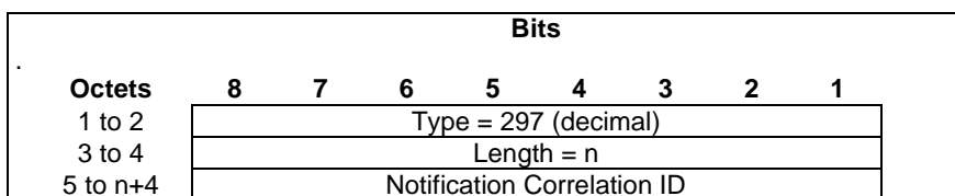
Figure 8.2.203-1: Notification Correlation ID
