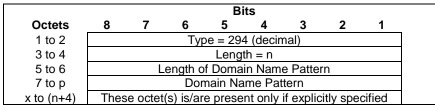
Figure 8.2.201-1: DNS Query Filter
