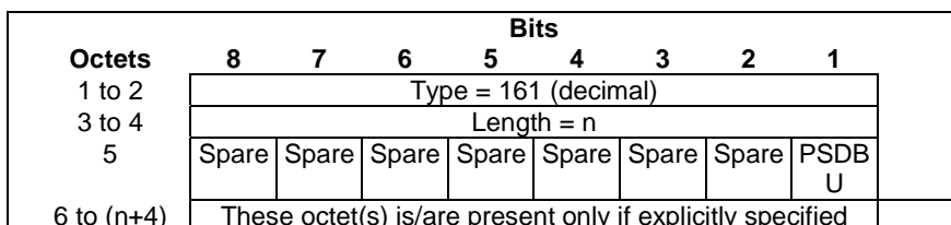
Figure 8.2.199-1: PFCPSRReq-Flags
