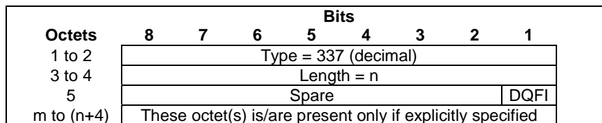
Figure 8.2.231-1: Measurement Indication IE
