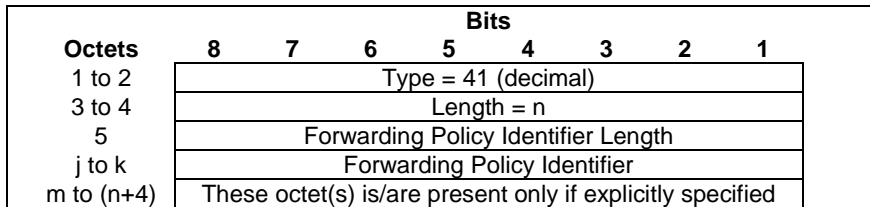
Figure 8.2.23-1: Forwarding Policy
