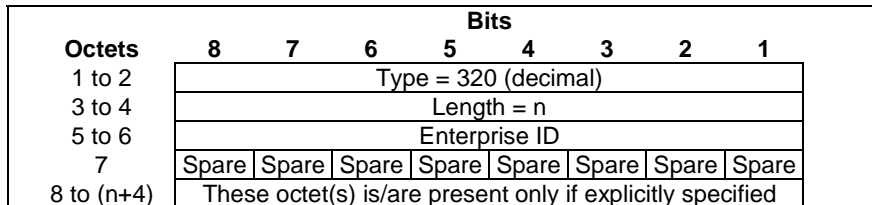
Figure 8.2.217-1: Vendor-Specific Node Report Type
