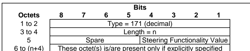
Figure 8.2.124-1: Steering Functionality
