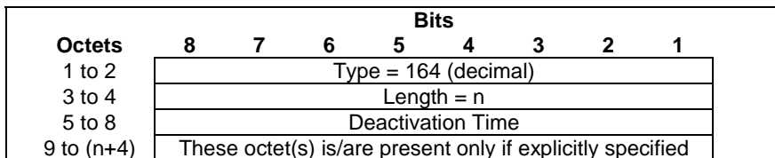
Figure 8.2.122-1: Deactivation Time
