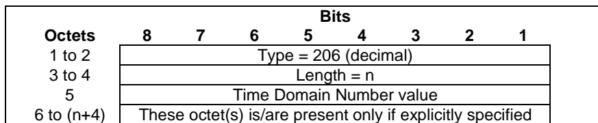
Figure 8.2.146-1: Time Domain Number
