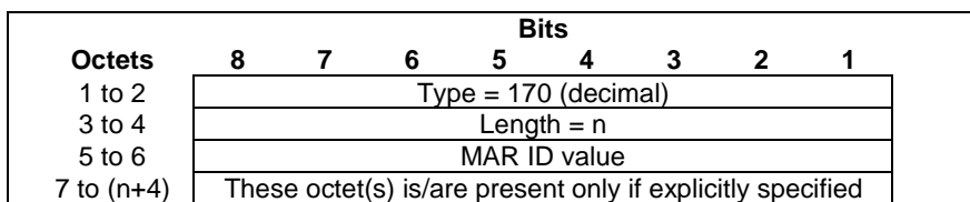
Figure 8.2.123-1: MAR ID
