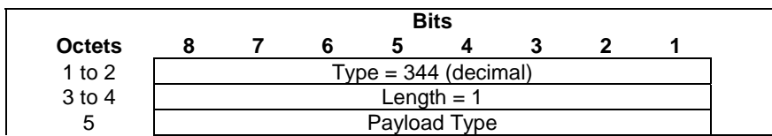
Figure 8.2.236-1: RTP Payload Type
