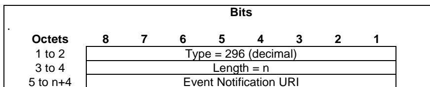
Figure 8.2.202-1: Event Notification URI
