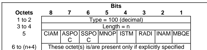
Figure 8.2.68-1: Measurement Information
