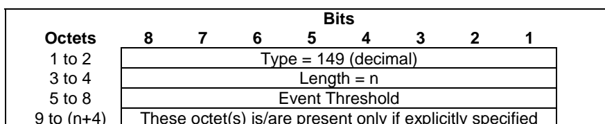
Figure 8.2.113-1: Event Threshold
