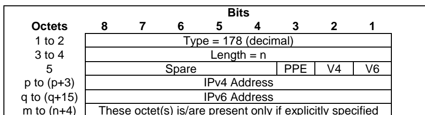
Figure 8.2.129-1: Alternative SMF IP Address
