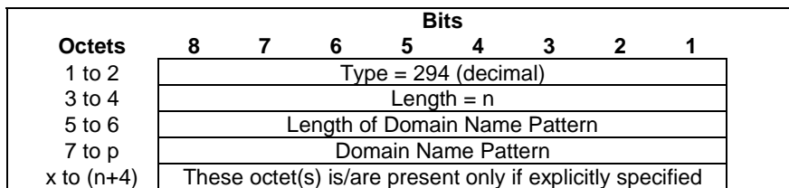
Figure 8.2.201-1: DNS Query/Response Filter
