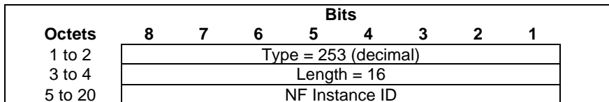
Figure 8.2.175-1: NF Instance ID
