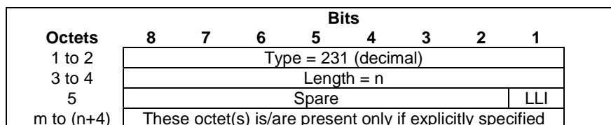
Figure 8.2.160-1: ATSSS-LL Information
