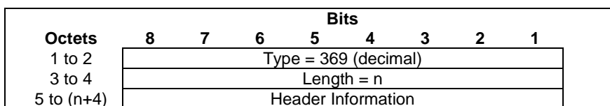
Figure 8.2.256-1: Header Information
