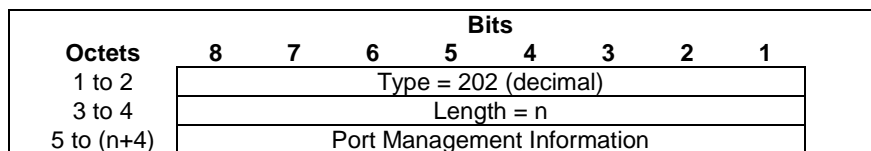
Figure 8.2.144-1: Port Management Information Container
