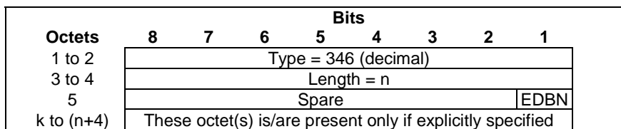
Figure 8.2.238-1: Extended DL Buffering Notification Policy
