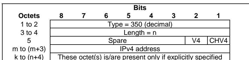
Figure 8.2.242-1: Mapped N6 IP Address
