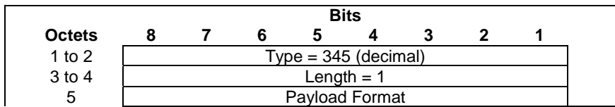
Figure 8.2.237-1: RTP Payload Format
