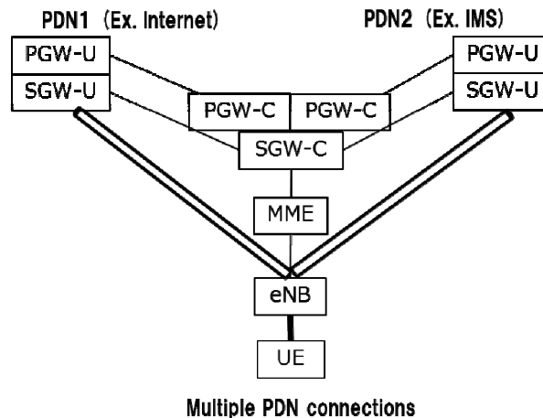
Figure B.2.4-1: SGW-U/PGW-U collocation with Control and User Plane Separation
