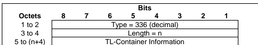
Figure 8.2.230-1: TL-Container
