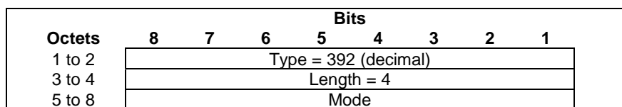
Figure 8.2.275-1: Security Mode (OWAMP or TWAMP)
