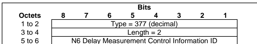
Figure 8.2.264-1: N6 Delay Measurement Control Information ID
