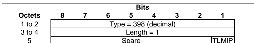
Figure 8.2.280-1: Transport Level Marking Indications
