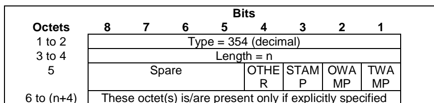
Figure 8.2.246-1: N6 Delay Measurement Protocols
