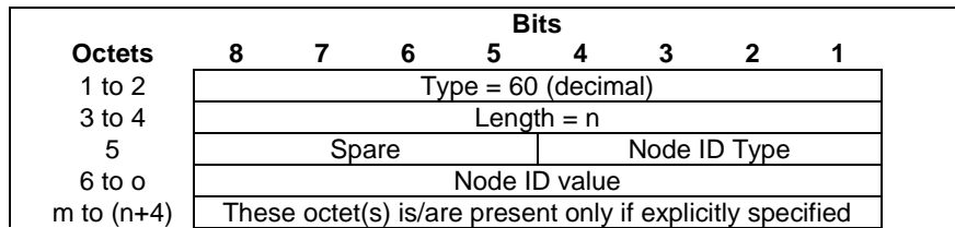
Figure 8.2.38-1: Node ID
