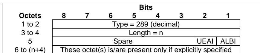
Figure 8.2.197.-1: Steering Mode Indicator
