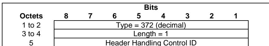
Figure 8.2.259-1: Header Handling Control ID
