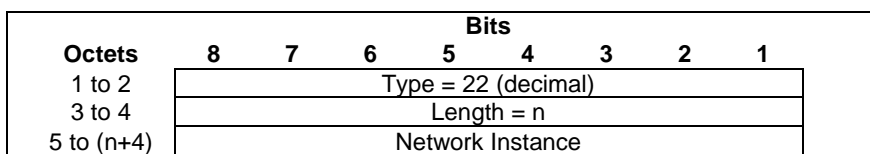
Figure 8.2.4-1: Network Instance
