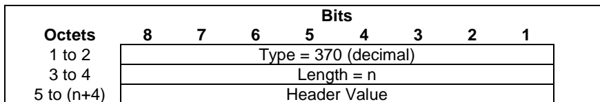
Figure 8.2.257-1: Header Information
