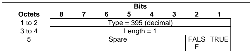
Figure 8.2.278-1: Expedited Transfer Indication
