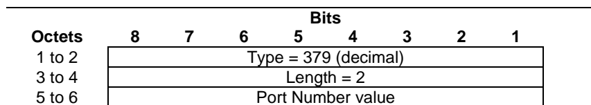
Figure 8.2.265-1: Measurement Endpoint Port Number
