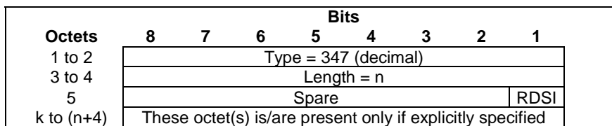
Figure 8.2.239-1: MT-SDT Control Information
