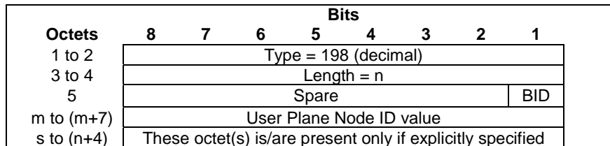
Figure 8.2.143-1: 5GS User Plane Node ID
