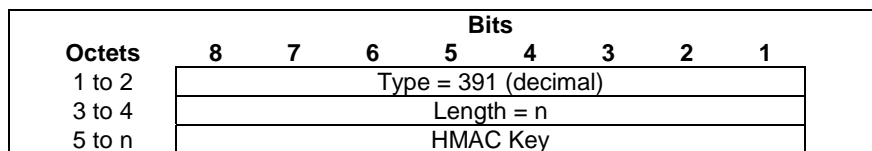
Figure 8.2.274-1: HMAC Key (STAMP)
