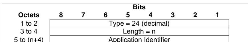
Figure 8.2.6-1: Application ID
