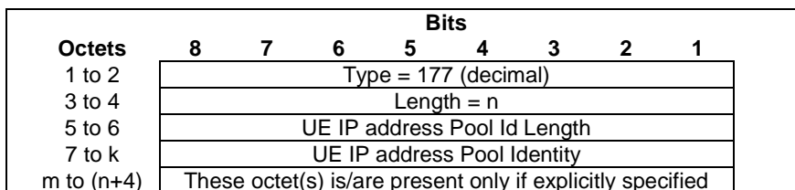
Figure 8.2.128-1: UE IP address Pool Identity
