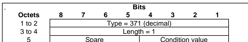
Figure 8.2.258-1: Header Handling Condition
