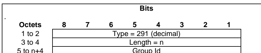
Figure 8.2.198-1: Group Id
