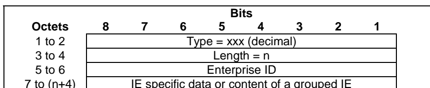
Figure 8.1.1-3: Vendor-Specific Information Element Format
