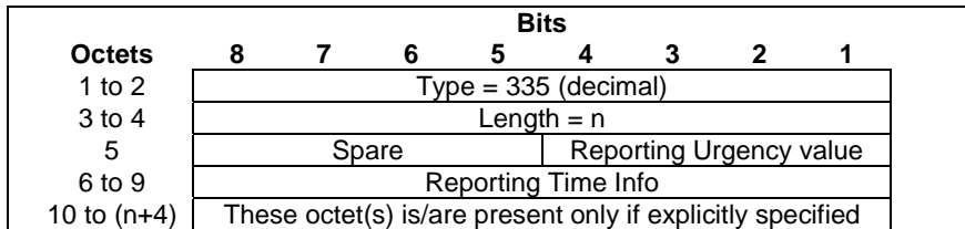
Figure 8.2.229-1: Reporting Suggestion Info
