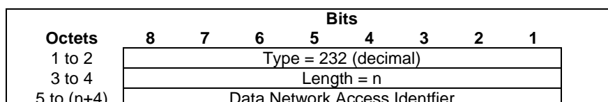
Figure 8.2.161-1: Data Network Access Identifier
