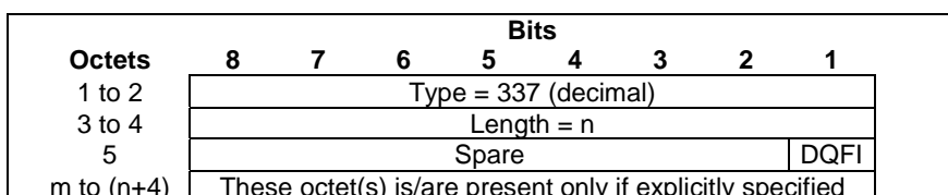
Figure 8.2.231-1: Measurement Indication
