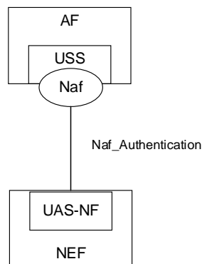
Figure 4.2.1.2-1: Reference architecture for Naf_Authentication service: SBI representation
