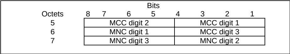
Figure 8.50-2: PLMN ID Parameter with 3-digit MNC
