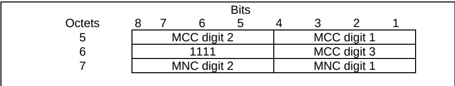
Figure 8.50-3: PLMN ID Parameter with 2-digit MNC
