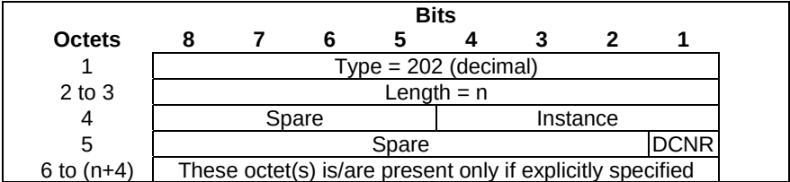
Figure 8.133-1: UP Function Selection Indication Flags
