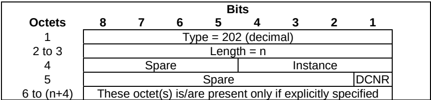
Figure 8.133-1: UP Function Selection Indication Flags
