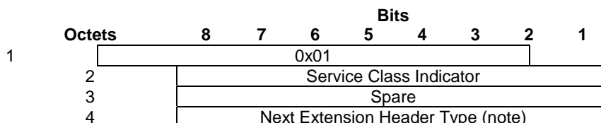
Figure 5.2.2.3-1: Service Class Indicator Extension Header
