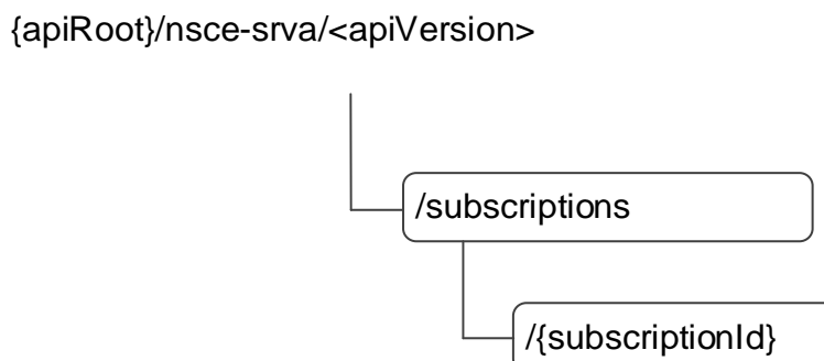
Figure 6.15.3.1-1: Resource URIs structure of the NSCE_SliceReqVerifyAndAlign API
