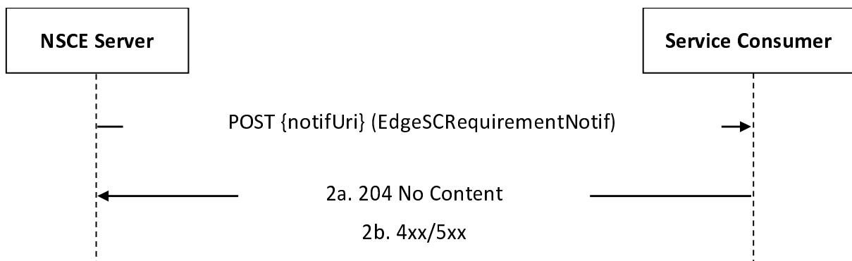
Figure 5.9.2.3.2-1: Edge service continuity requirement Notification
