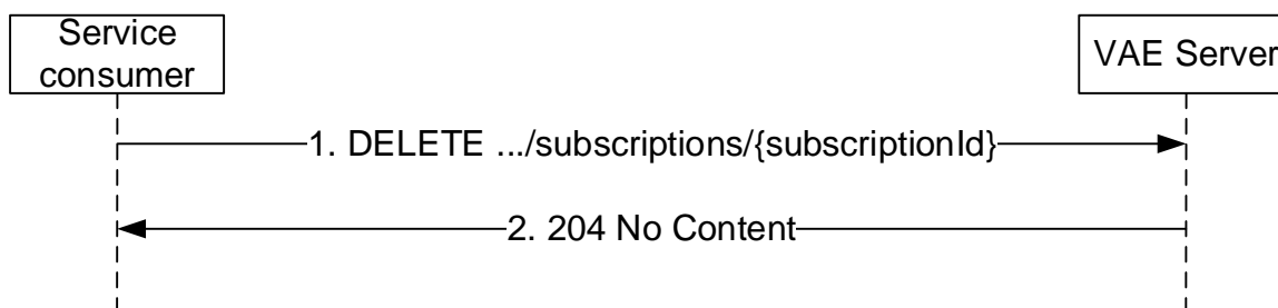
Figure 5.8.2.6.2-1: Terminate Session
