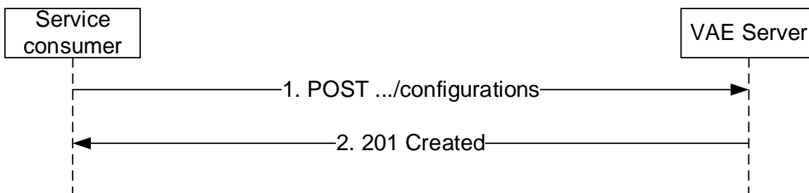
Figure 5.9.2.2.2-1: Request_V2VConfigRequirement
