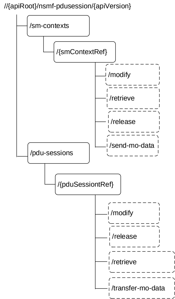
Figure 6.1.3.1-1: Resource URI structure of the Nsmf_PDUSession API
