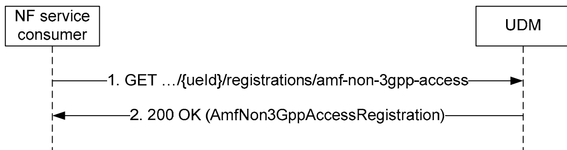
Figure 5.3.2.5.3-1: Requesting a UE's AMF Registration Information for non-3GPP Access
