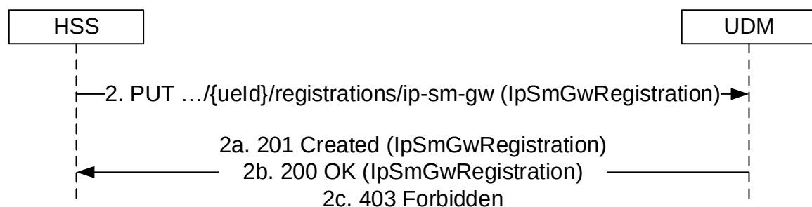
Figure 5.3.2.2.7-1: IP-SM-GW registration
