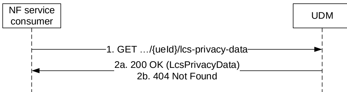
Figure 5.2.2.15-1: Requesting a UE's LCS Privacy Data
