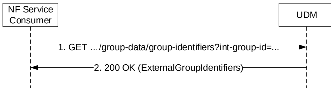
Figure 5.2.2.14-2: Internal Group Identifier Translation
