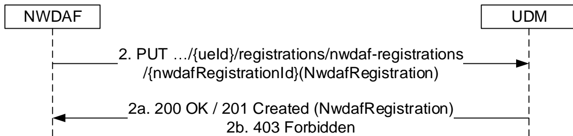
Figure 5.3.2.2.8-1: NWDaf registration
