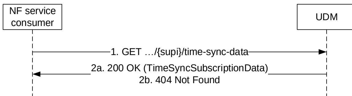
Figure 5.2.2.2.26-1: Requesting a UE's Time Synchronization Subscription Data
