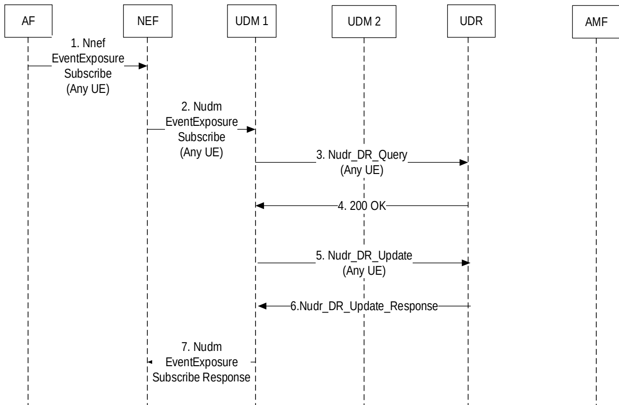
Figure B-4: Any UE Subscription
