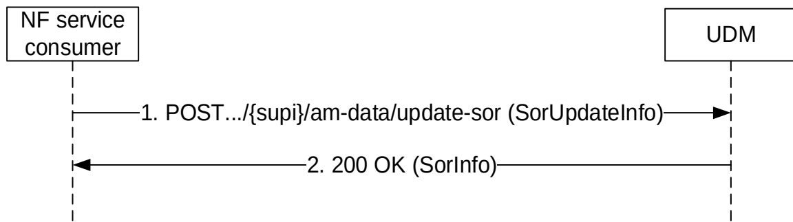
Figure 5.2.2.6-1: Triggering update of Steering Of Roaming information
