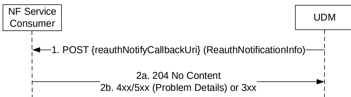
Figure 5.3.2.15.2-1: Reauthentication Notify
