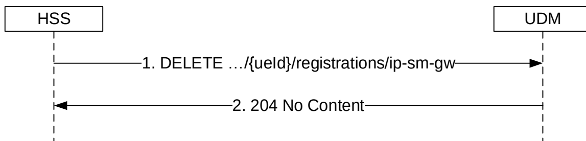
Figure 5.3.2.4.7-1: IP-SM-GW deregistration
