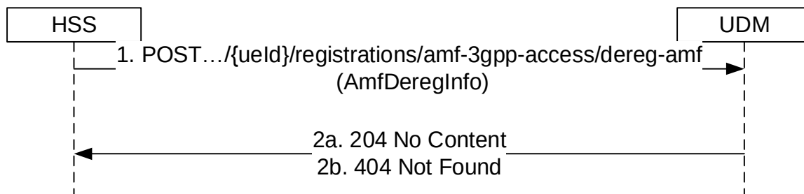
Figure 5.3.2.9.2-1: AMF-Deregistration
