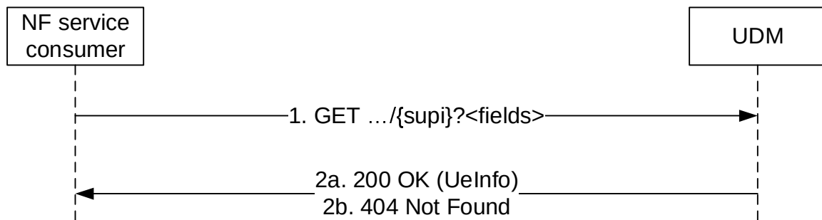
Figure 5.8.2.2-1: NF service consumer requesting domain selection information
