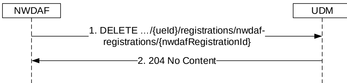
Figure 5.3.2.4.8-1: NWDAF deregistration
