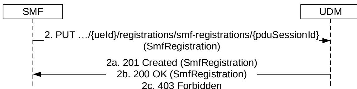
Figure 5.3.2.2.4-1: SMF registration
