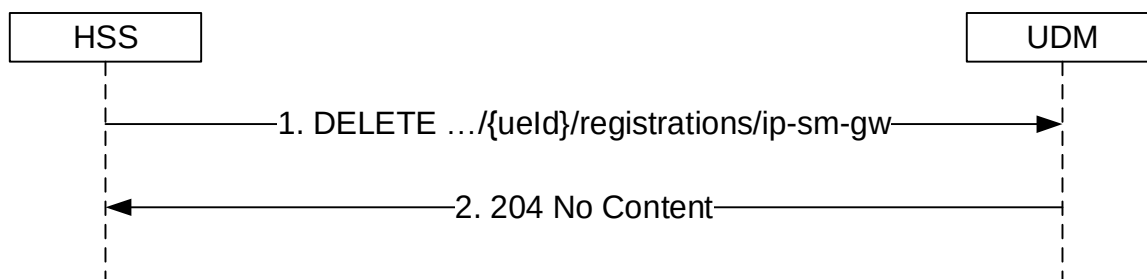
Figure 5.3.2.4.7-1: IP-SM-GW deregistration
