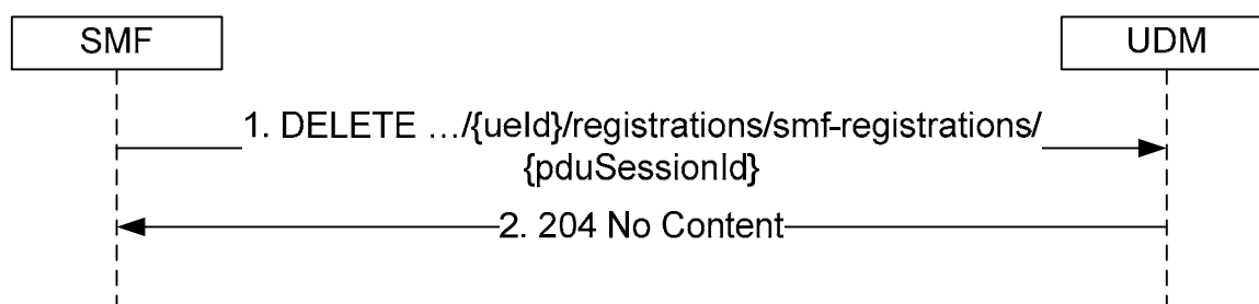
Figure 5.3.2.4.4-1: SMF deregistration
