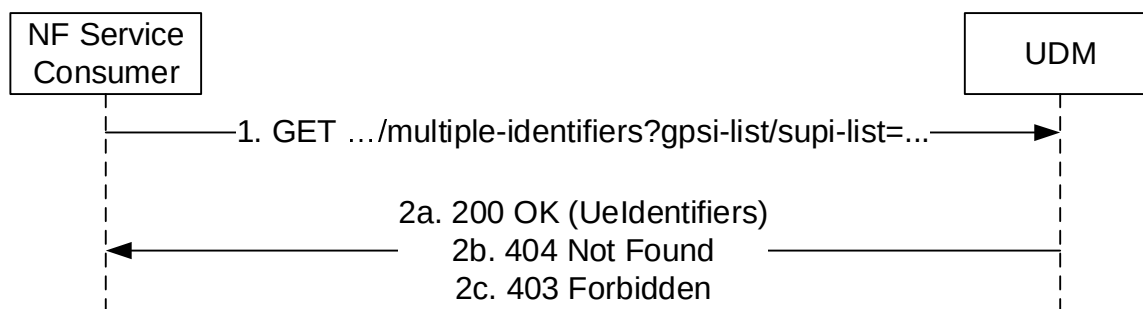
Figure 5.2.2.2.25: GPSIs/SUPIs Translation
