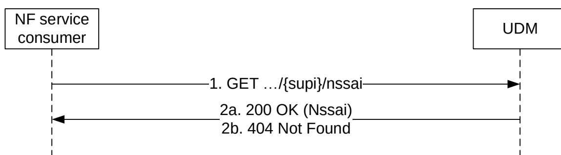
Figure 5.2.2.2.2-1: Requesting a UE's NSSAI
