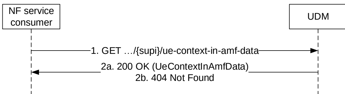
Figure 5.2.2.2.20-1: Requesting a UE's Context in AMF Data
