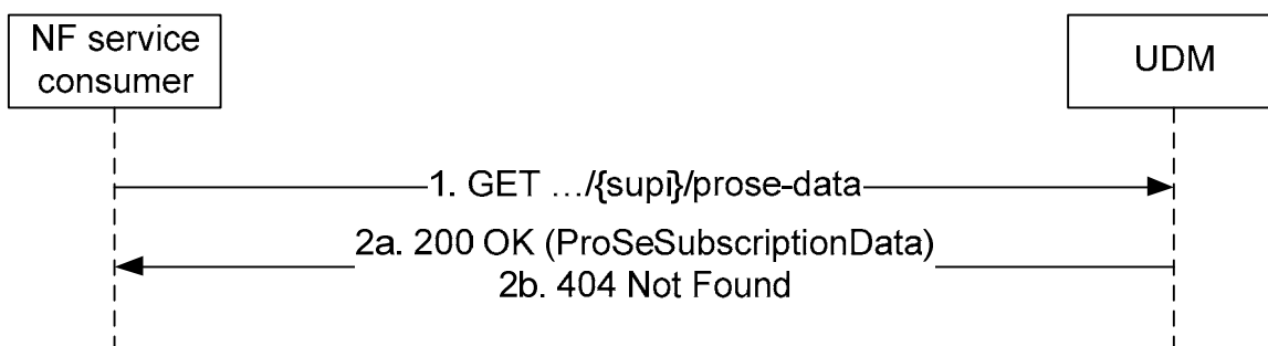
Figure 5.2.2.2.22-1: Requesting a UE's ProSe Subscription Data
