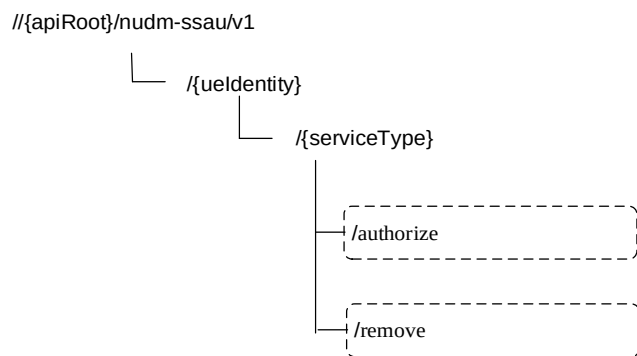
Figure 6.8.3.1-1: Resource URI structure of the Nudm-SSAU API
