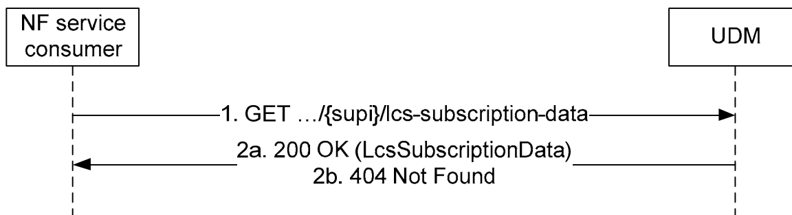
Figure 5.2.2.27-1: Requesting a UE's LCS Subscription Data
