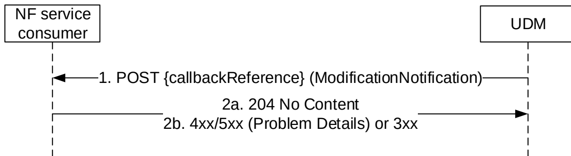
Figure 5.2.2.5.2-1: Subscription Data Change Notification
