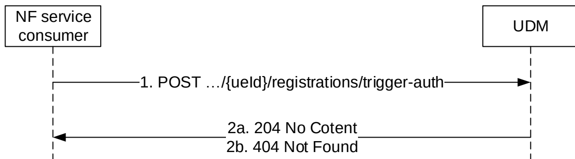
Figure 5.3.2.16.2-1: Auth Trigger
