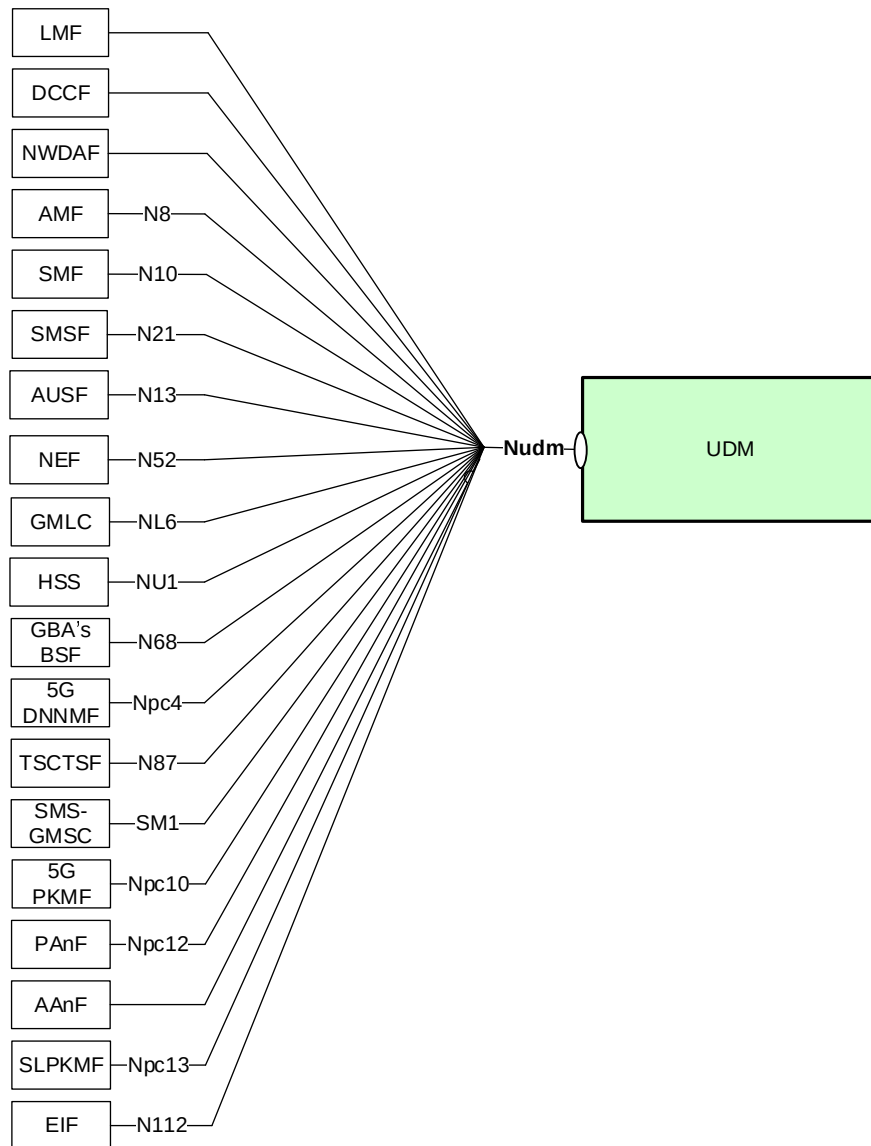
Figure 4.1-1: Reference model – UDM
