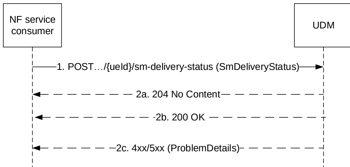
Figure 5.10.2.2-1: Report the SM-Delivery Status
