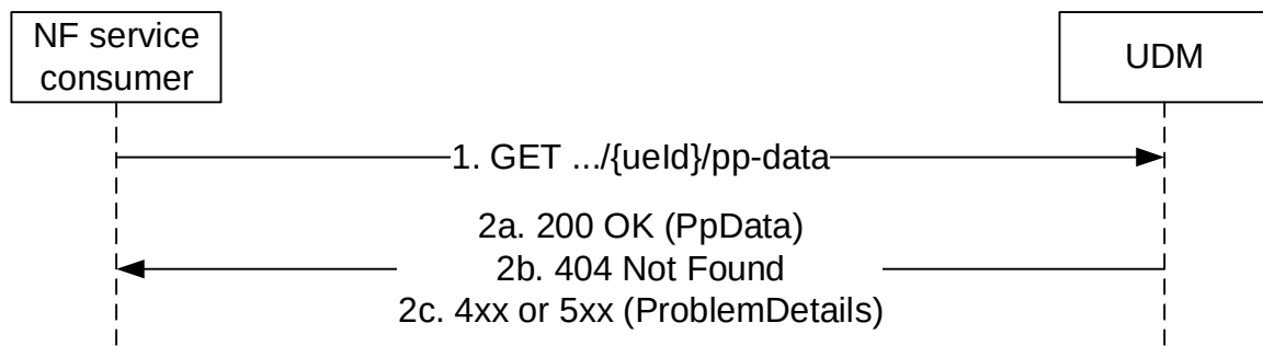
Figure 5.6.2.5.5-1: NF service consumer gets Parameter Provisioning Data
