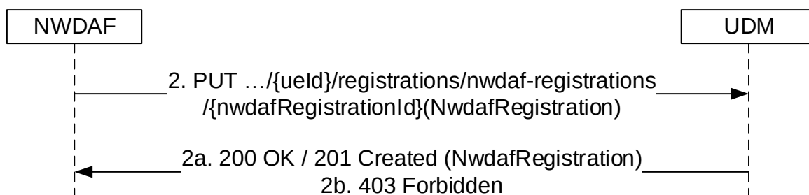
Figure 5.3.2.2.8-1: NWDAF registration
