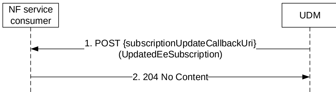
Figure 5.5.2.4.5-1: Subscription Update Notification
