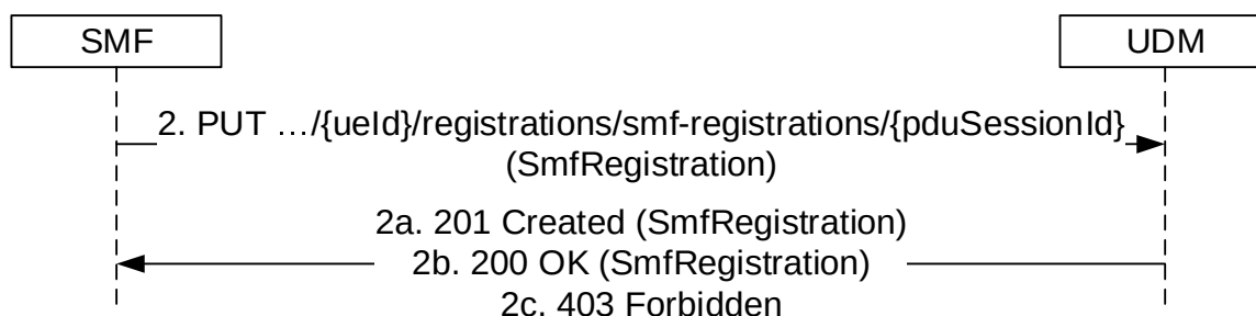
Figure 5.3.2.2.4-1: SMF registration
