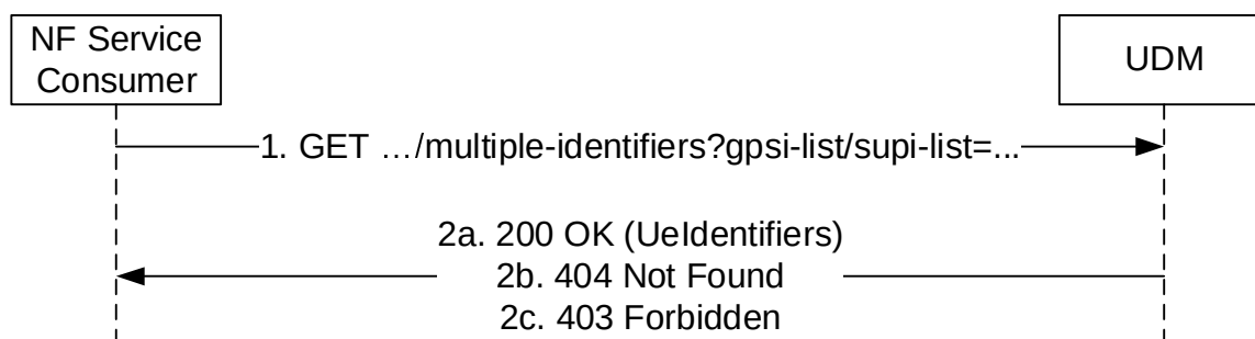
Figure 5.2.2.25: GPSIs/SUPIs Translation
