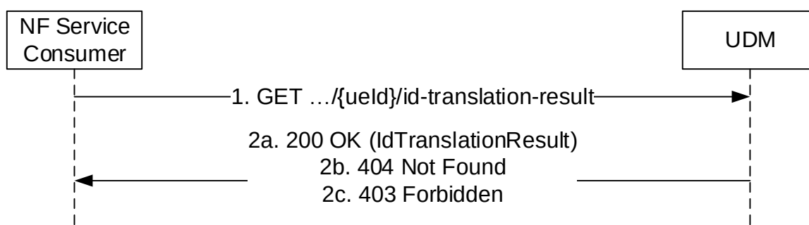
Figure 5.2.2.2.10-1: Identifier Translation
