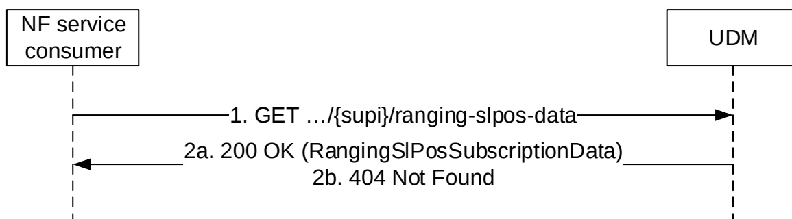
Figure 5.2.2.28-1: Requesting a UE's Ranging and Sidelink Positioning Subscription Data
