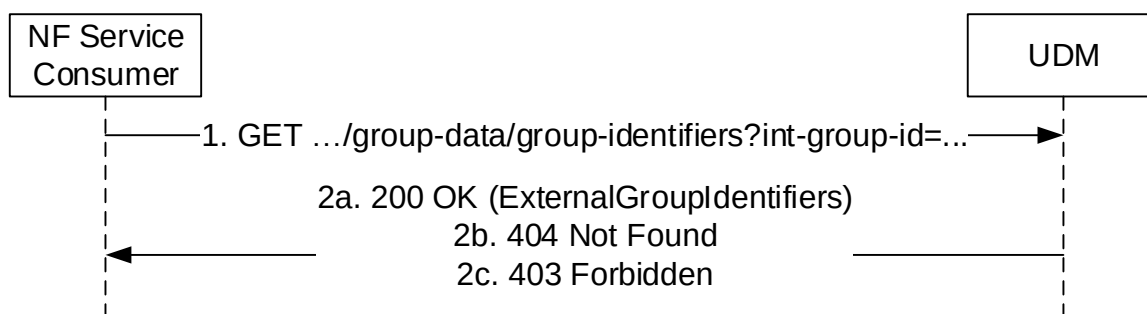
Figure 5.2.2.14-2: Internal Group Identifier Translation
