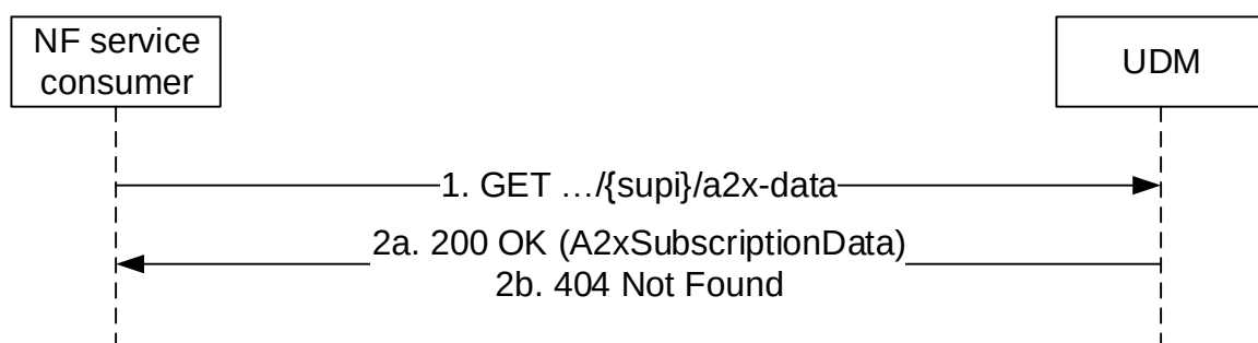
Figure 5.2.2.29-1: NF service consumer retrieves A2X Subscription Data
