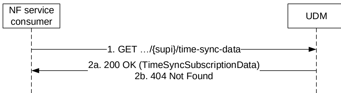
Figure 5.2.2.26-1: Requesting a UE's Time Synchronization Subscription Data
