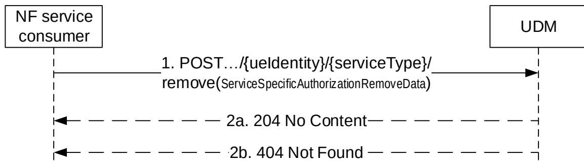
Figure 5.9.2.4.2-1: Service Specific Authorization Data Removal
