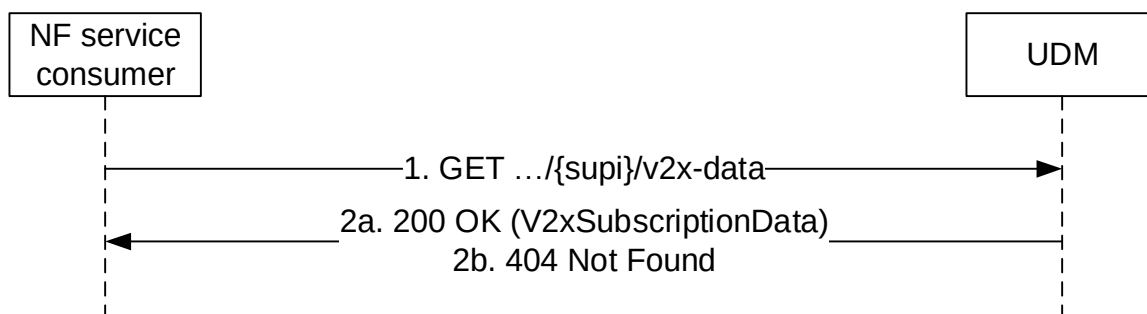
Figure 5.2.2.18-1: NF service consumer retrieves V2X Subscription Data
