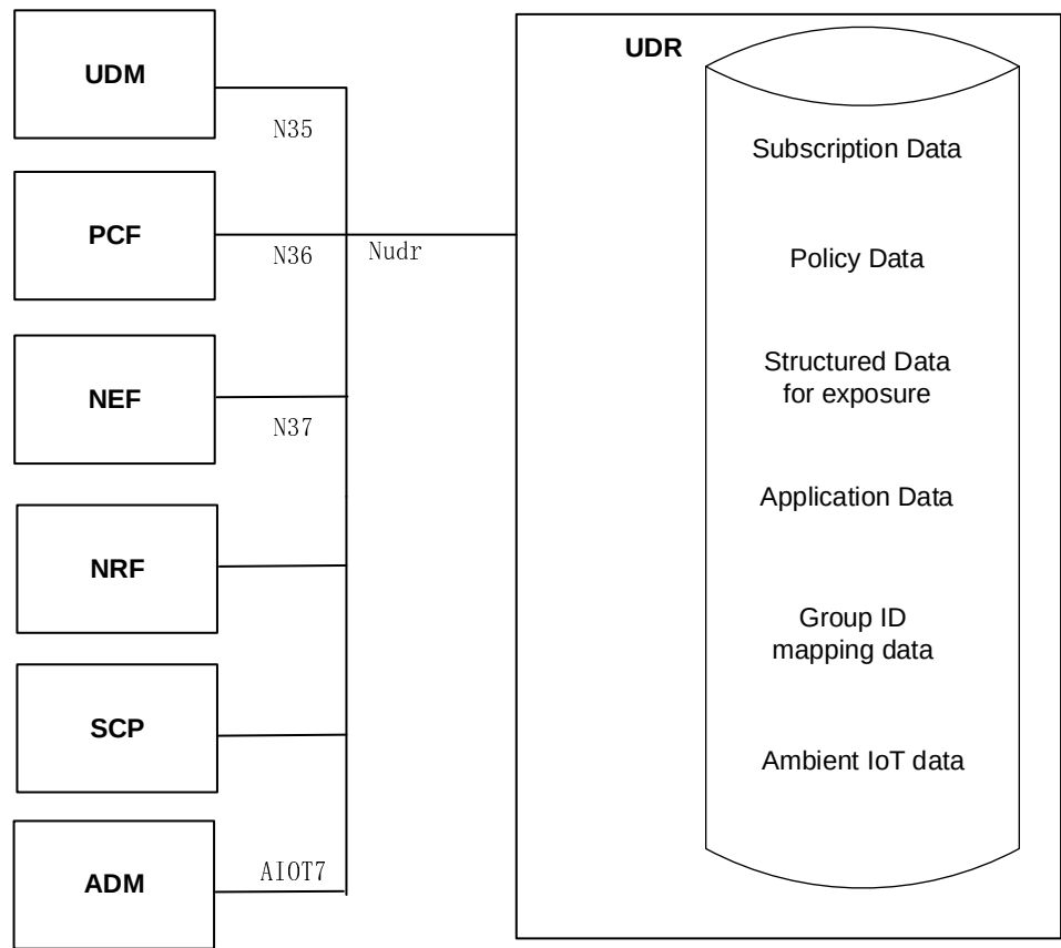
Figure 4-1: Data storage architecture
