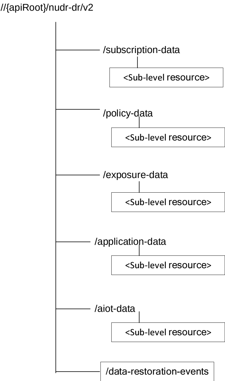
Figure 6.1.3.1-1: Resource URI structure of the Nudr_DataRepository API
